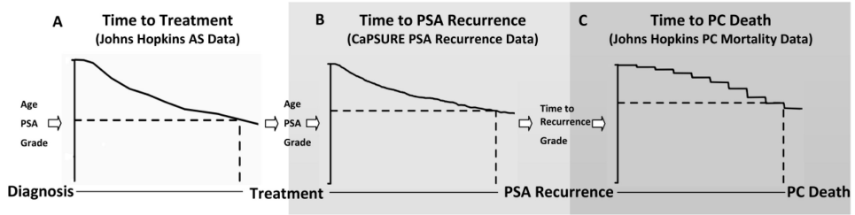
Figure 1. Framework for modeling of prostate cancer mortality following active surveillance versus immediate radical prostatectomy. Under immediate treatment, we model time to recurrence (B) followed by time from recurrence to prostate cancer mortality (C). Under active surveillance, these are preceded by a model of time to treatment (A). The figures show Kaplan-Meier curves for the relevant endpoints from the three data sets used in the model.
