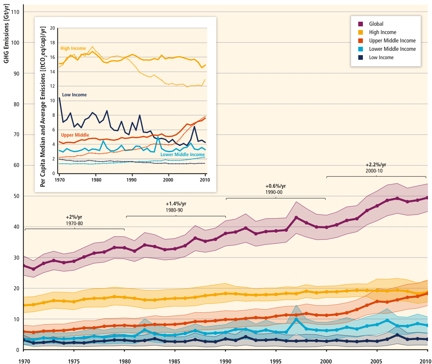
Figure 1.4 | Global growth in emissions of GHGs by economic region. Main figure shows world total (top line) and growth rates per decade, as well as the World Bank's four economic regions (see Figure 1.1 caption for more detail). Inset shows trends in annual per capita mean (solid lines) and median (dotted lines) GHG emissions by region 1970–2010 in tonnes of CO 2 eq (t/cap/yr) (United Nations, 2013a). Global totals include bunker fuels; regional totals do not. The data used is from the same sources reported in Figure 1.3c. Error bars are approximated confidence interval of 1 standard deviation, derived by aggregating individual country estimates by gas and sector of the 16th and 84th emission percentiles provided by the MATCH analysis (Höhne et al., 2011); data also available at http://www.match-info.net/ . However, we note that this probably over-states actual uncertainty in the totals, since individual country uncertainty estimates under this method are implicitly taken to be completely correlated. Thus, for the global totals we estimate a 90% uncertainty range using the same method as discussed for Figure 1.3c. While in 2010 the uncertainty using that method is 9%, over the full time period of Figure 1.4 the value varies from 9% to 12% with an average value of 10%. We caution that multi-country and global uncertainty estimates remain an evolving area of research (see caption 1.3c and Section 5.2.3). Uncertainties shown on this chart are at best indicative of the unknowns but are not a definitive assessment.
