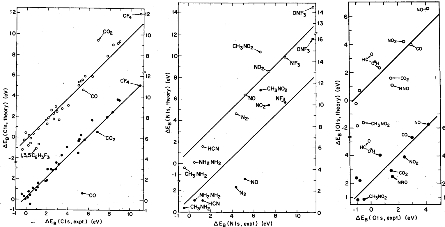
Fig. 7. This illustrates the "blanket" approach toward predicting chemical shifts. Both the ground state model (in filled circles) and the relaxation model (in open circles) are presented. The lines represent best least-squares fits of experiment to theory under the constraint of unit slope. The standard deviations are given in Ref. 26.
