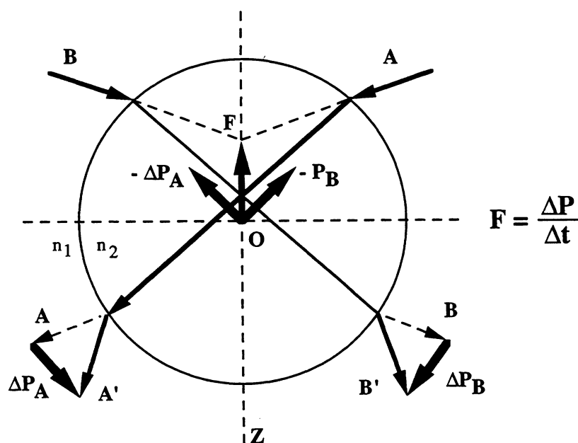
Fig. 1 Single-beam gradient force optical trap. Transverse, as well as axial forces, pull the polarized dielectric cell towards the beam spot.
