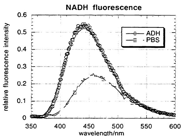
Fig. 5a Fluorescence of free 0.1 mM NADH and bound NADH (NADH-ADH mixture) in PBS
