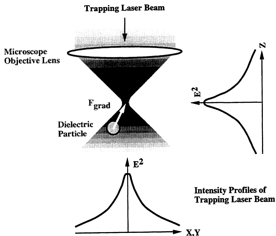
Fig. 1 Single-beam gradient force optical trap. Transverse, as well as axial forces, pull the polarized dielectric cell towards the beam spot.
