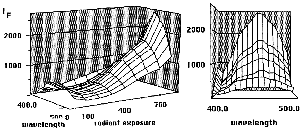
Fig. 8 Modifications of the autofluorescence spectrum of a single cell during UVA exposure. Plots contain data of spectrum 1 (1 J/cm 2 ), 101, 201, 301, 401, 501, 601, 701, and 801 (801 J/cm 2 ). Spectrum 801 was obtained after a dark phase of 10 min.
