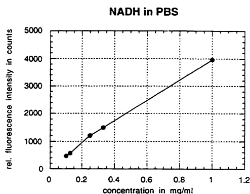
Fig. 5b Fluorescence intensity of free NADH in dependence on concentration. Background intensity (PBS-filled chamber): 2000 \pm 100 counts.
