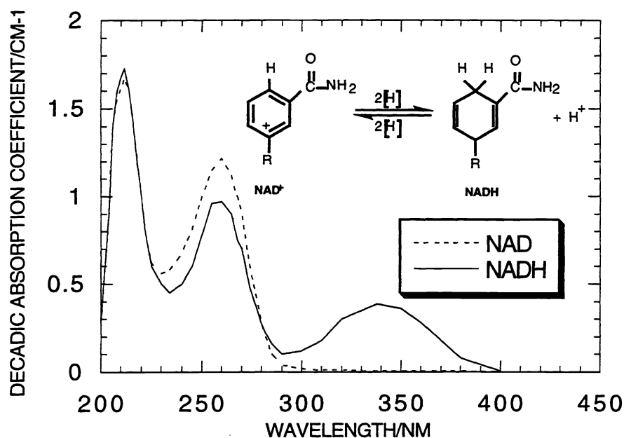
Fig. 3 Structure and absorption spectra of NAD/NADH (64 \mu M, PBS)
