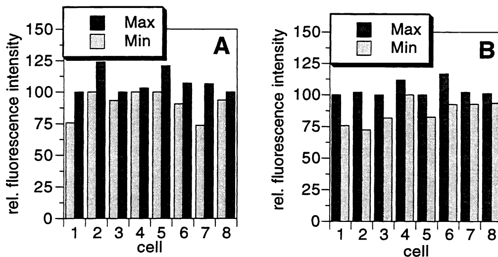
Fig. 6. Relative fluorescence extrema of cells trapped for 20 min (A) compared with control (B).
