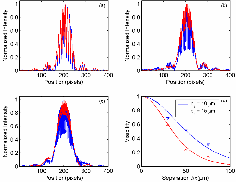
Fig. 3. (a-c) Interference fringes with average visibility (red), obtained by integrating the whole interferogram, and fringes with highest visibility (blue), picked by manually scanning the interferogram. For comparison the fringe patterns are normalized in intensity and overlap each other. The slit separations are (a) 30, (b) 50, and (c) 75 μm. (d) Experimental data ( \Delta, \nabla ) of fringe visibilities at different slit separations and theoretical predictions based on van Cittert-Zernike theorem. The source size is 10 μm (blue, corresponding to highest visibilities in (a-c)) and 15 μm (red, corresponding to average visibilities).
