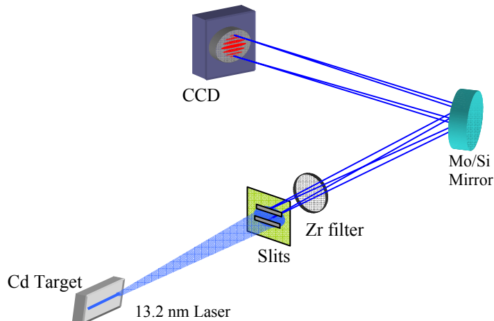
Fig. 1. Young's double-slit experiment setup for measuring the spatial coherence of a 13.2 nm soft x-ray laser.
