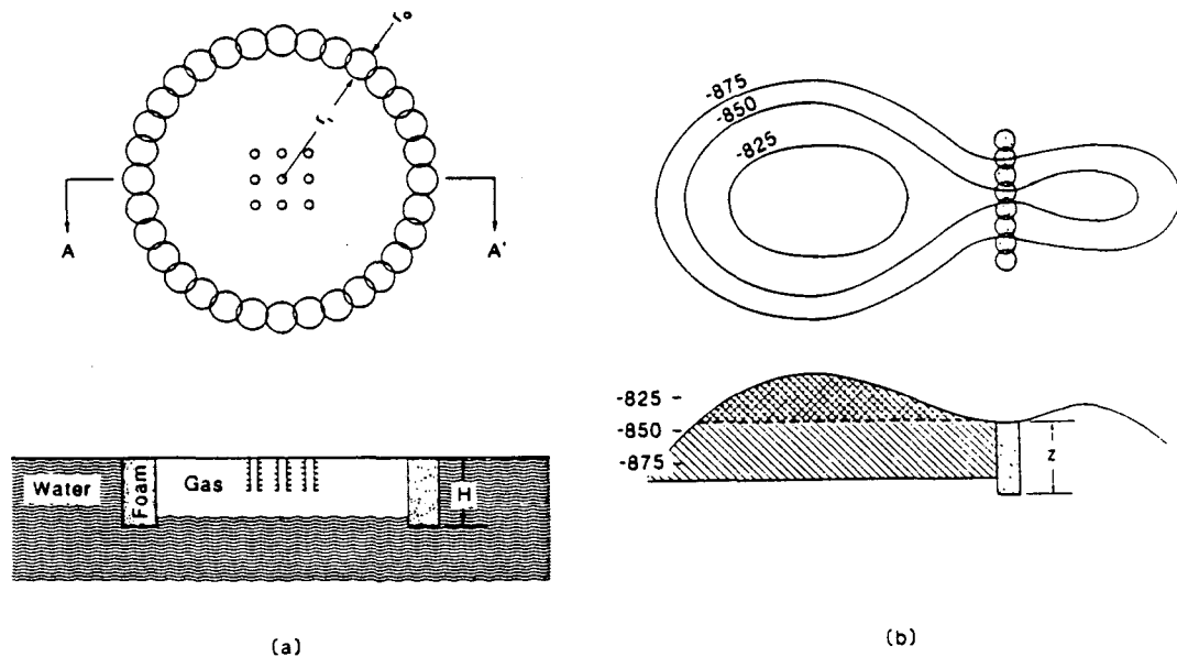
Figure 1. Application of foam to improve underground gas storage by controlling gas migration (after Witherspoon et al., 1987). (a) Foam plumes formed at peripheral wells intersect to form a continuous barrier, containing stored gas in a more compact bubble near the injection-withdrawal wells. The use of foam obviates the need for natural closure. (b) A small foam barrier to cut off a spill point produces a large increase in storage capacity.
