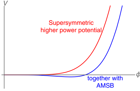
FIG. 2. Schematics of the potential for s -confining and free magnetic phases. The red curve is for SQCD with power-law behavior, while the blue curve for ASQCD has a well-defined minimum.
