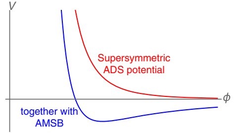
FIG. 1. Schematics of the potential for N_f < N_c . The red curve is for SQCD with runaway behavior, while the blue curve for ASQCD has a well-defined minimum.
