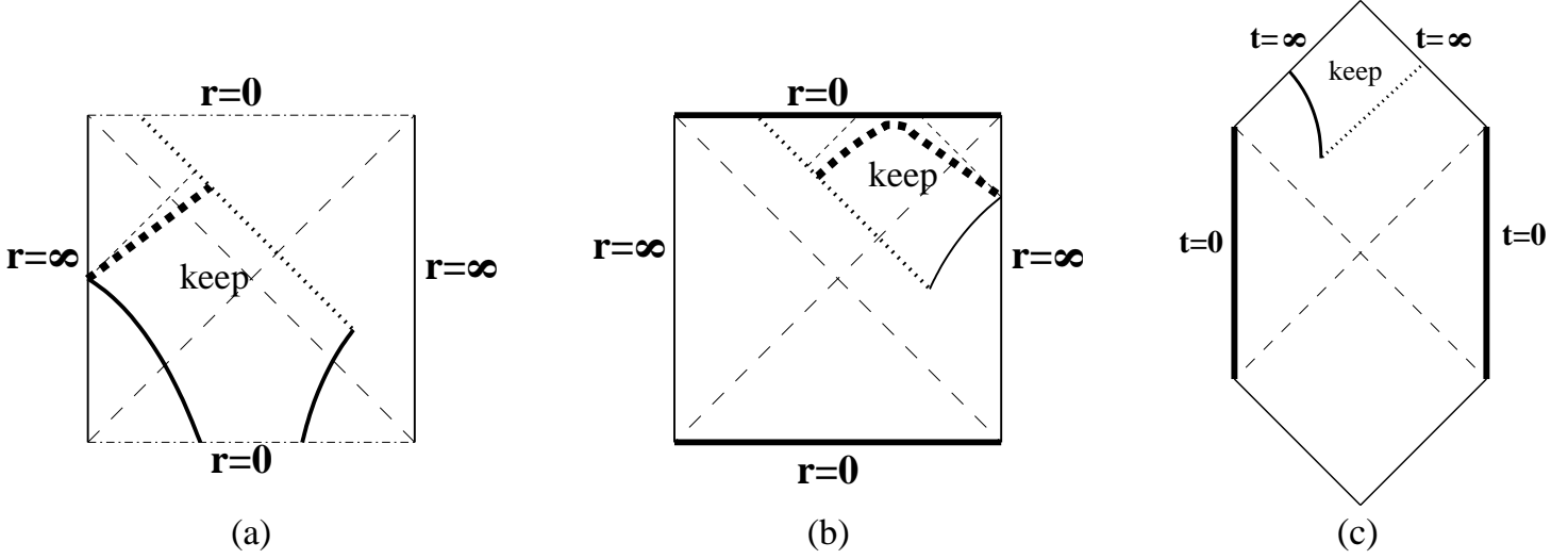
Fig. 6: The full diagram, Fig. 5, is constructed from the pieces shown here. In the thin wall approximation, (a) is the conformal diagram for AdS spacetime in H_2 slicing. The top and bottom dot-dashed lines are coordinate singularities where the size of the H_2 goes to zero. The region we use, labelled “keep” in the figure, is bounded by the domain wall (heavy curved lines) and the shell of radiation emitted from the collision (dotted line). As described in the text, the thin wall solution has a Cauchy horizon (thin, short dashes). Going beyond the thin wall approximation, the Cauchy horizon will be removed by a spacelike curvature singularity (heavy dashed line). Diagram (b) is the hyperbolic AdS black hole. The region we use is bounded by the null shell of radiation and the domain wall. The curvature singularity of (a) must continue across the null shell into (b). Just as in (a), a Cauchy horizon forms at the point where the domain wall hits the boundary, so again a curvature singularity must cut off the boundary at the point where the domain wall hits it. Diagram (c) is the hyperbolic \Lambda = 0 solution, bounded by the domain wall and the null shell radiated into the \Lambda = 0 side of the domain wall. Note that we do not use the part of the spacetime which contains timelike singularities.
