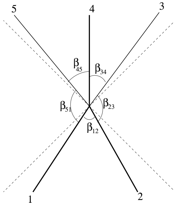
Fig. 12: The absence of a conical deficit at the collision point leads to a constraint on the relative boosts \beta of the colliding domain walls, equation (A.3).
