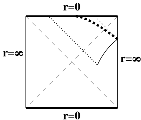
Fig. 4: If \kappa \neq 1/\ell , the domain wall accelerates out to infinity in finite time in the AdS-Schwarzschild black hole. As we explain later, we expect a singularity to form along the heavy dashed line.
