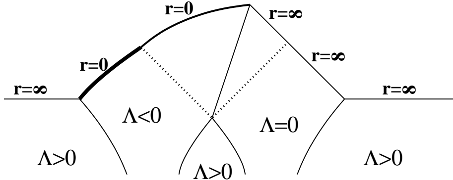
Fig. 8: Gluing Fig. 7 onto the asymptotically flat bubble yields a hyperbolic black hole with an asymptotically flat region of spacetime.
