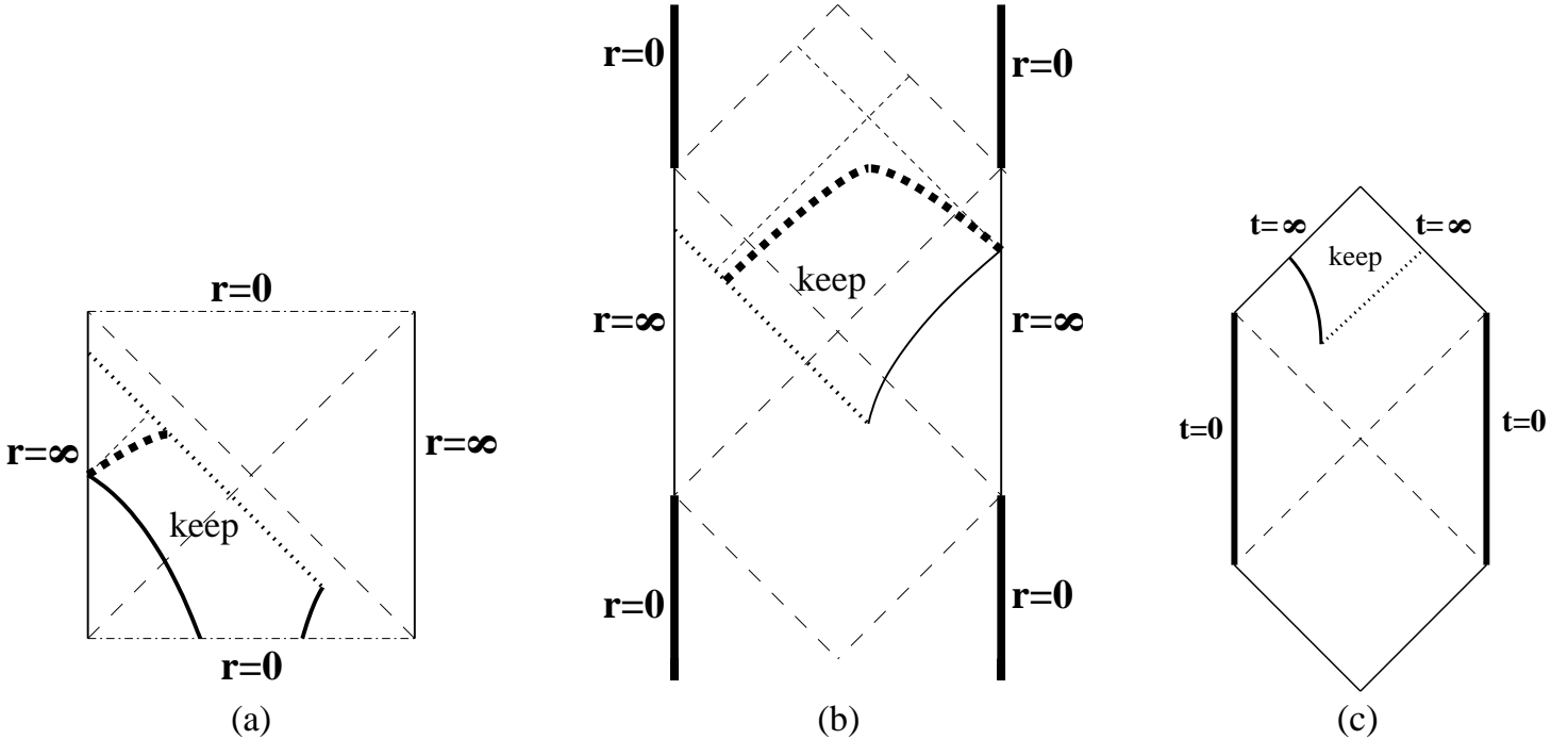
Fig. 9: In the case that the collision occurs on an H_2 with radius of curvature less than the AdS scale, the situation is slightly different from Fig. 6. In this case, the null shell of radiation on the \Lambda < 0 side of the domain wall ends up behind the white hole horizon. Also (b) is now a hyperbolic AdS black hole with negative M .
