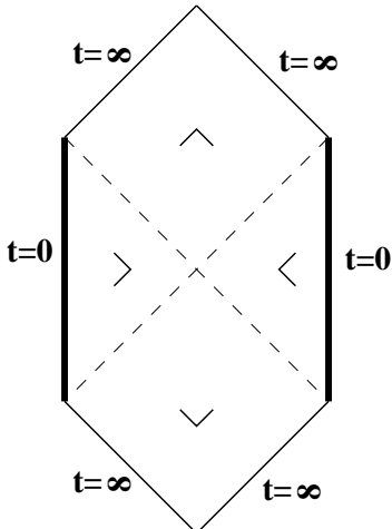
Fig. 2: The Penrose diagram for the “hyperbolic Schwarzschild” spacetime. Each point represents a hyperboloid and the singularities are timelike. We will only be interested in the region to the future of the surface t = t_0 (denoted by the dashed line), so these singularities will not enter our discussion. The “wedges” will be explained in section 2.5.
