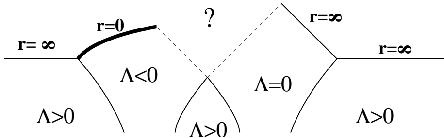
Fig. 1: Bubbles with zero and negative cosmological constant can collide. The heavy black line denotes the curvature singularity which always forms in the \Lambda < 0 bubble. The \Lambda = 0 bubble always includes a piece of future null infinity. We will investigate what happens to the future of the collision.
