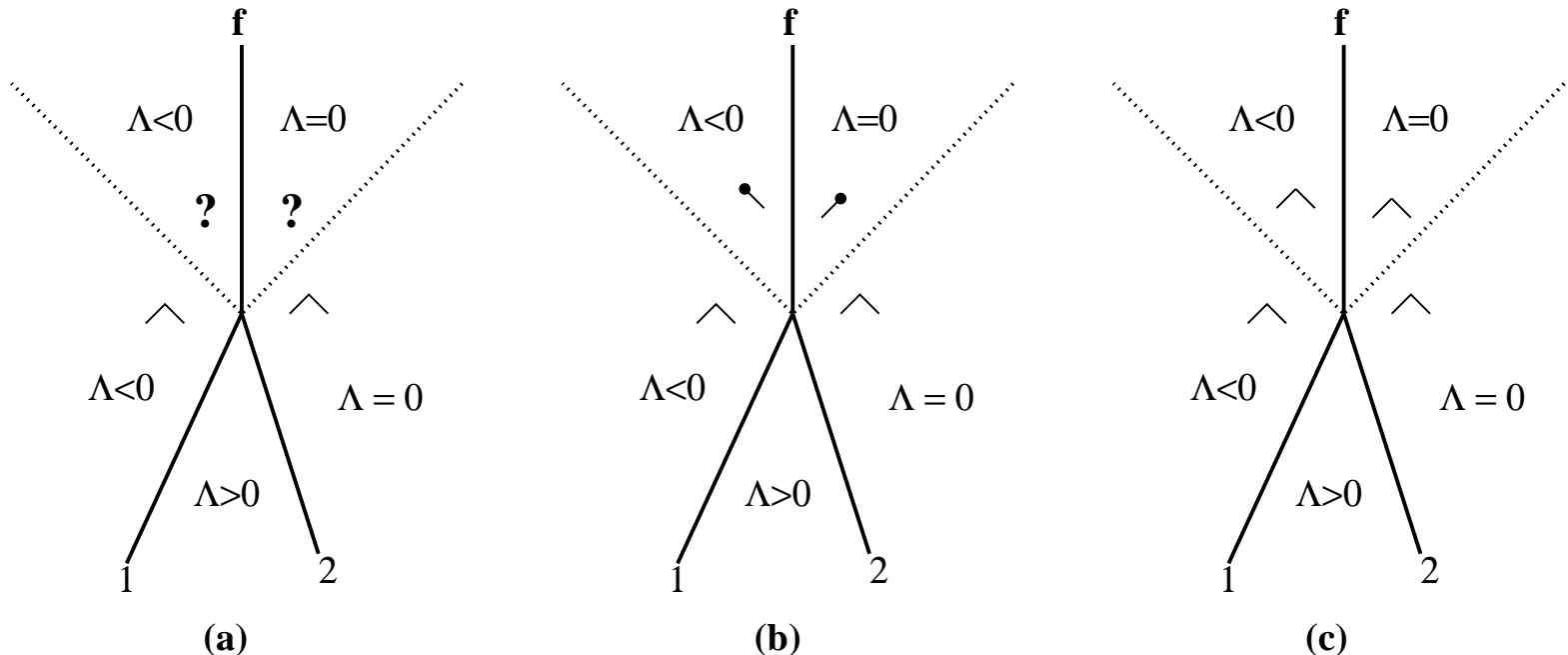
Fig. 11: This figure demonstrates how to determine the direction of the Bousso wedge in the spacetime to the future of the collision, when the collision happens at a radius R < \ell . Outside the future lightcone of the collision, the wedges have the behavior shown in Fig. 10. Inside the future lightcone, we do not know the direction yet, as shown in (a). Continuity of R across the null shell partly determines the behavior inside the future lightcone, as shown in (b). Here the dots denote the vertex of the wedge. Now imagine starting in the \Lambda = 0 region and following the known decreasing null ray across the final domain wall. This ray is left-moving and past-directed. R must continue to decrease along this ray after crossing the domain wall since we have assumed the null energy condition, so in the \Lambda < 0 region the left-moving past-directed ray must decrease. We can repeat the same argument reversing the two sides of the domain wall, leading to the final diagram (c).
