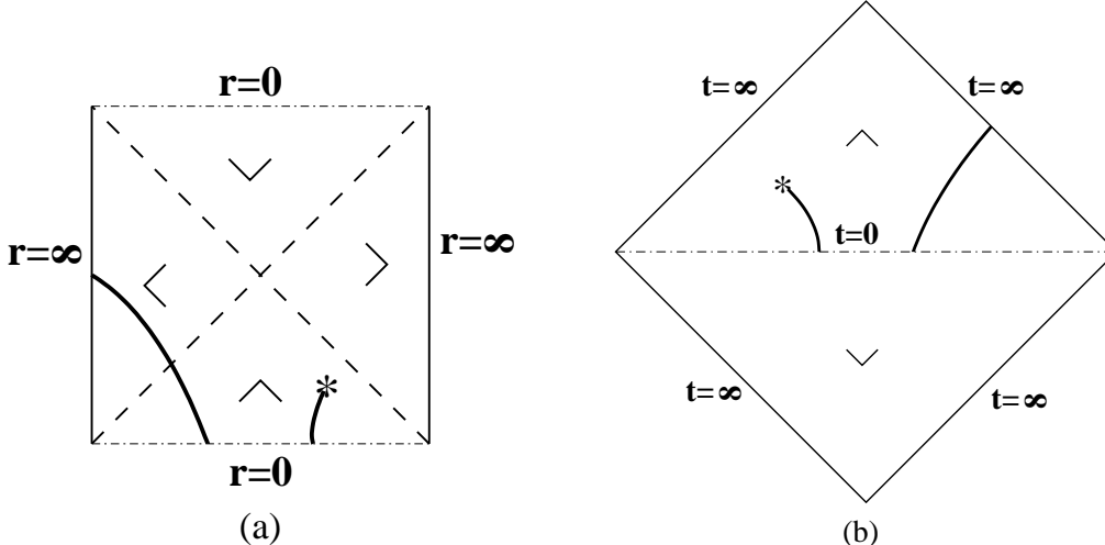
Fig. 10: “Bousso wedges” indicate in which null directions the curvature radius of the hyperboloids decreases. Figure (a) is a piece of AdS spacetime, while (b) is a piece of Minkowski spacetime. The collision occurs at the point marked with a star(*). When the collision occurs at R < \ell , it is “behind the horizon” in AdS, as shown in (a).
