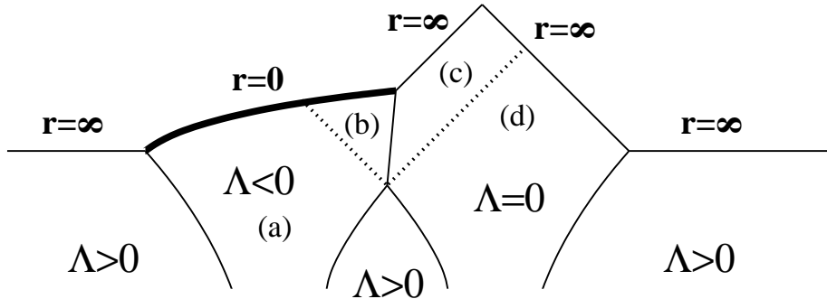
Fig. 5: A sketch of the conformal diagram for a collision in which the resulting domain wall has tension exceeding the BPS bound. In the thin wall approximation, region (a) is a piece of AdS spacetime, (b) is a piece of the hyperbolic AdS black hole, (c) is a piece of the hyperbolic Schwarzschild solution, while (d) is a piece of Minkowski spacetime. Going infinitesimally beyond the thin wall approximation results in additional singularities to create a diagram like the one shown here. In the next figure, we show the regions (a), (b), and (c) in more detail.
