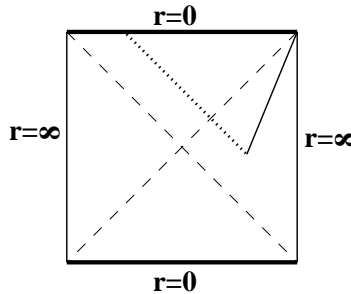
Fig. 7: If the tension saturates the BPS bound, the domain wall reaches infinity in infinite time outside the AdS-Schwarzschild black hole.
