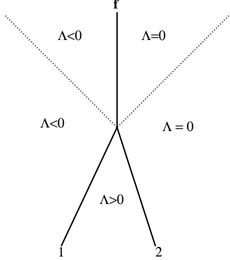
Fig. 3: In our thin wall approximation, the spacetime near the collision is divided into five regions. The dotted lines denote outgoing shells of radiation. The solid lines denote two incoming bubble walls and the outgoing domain wall.
