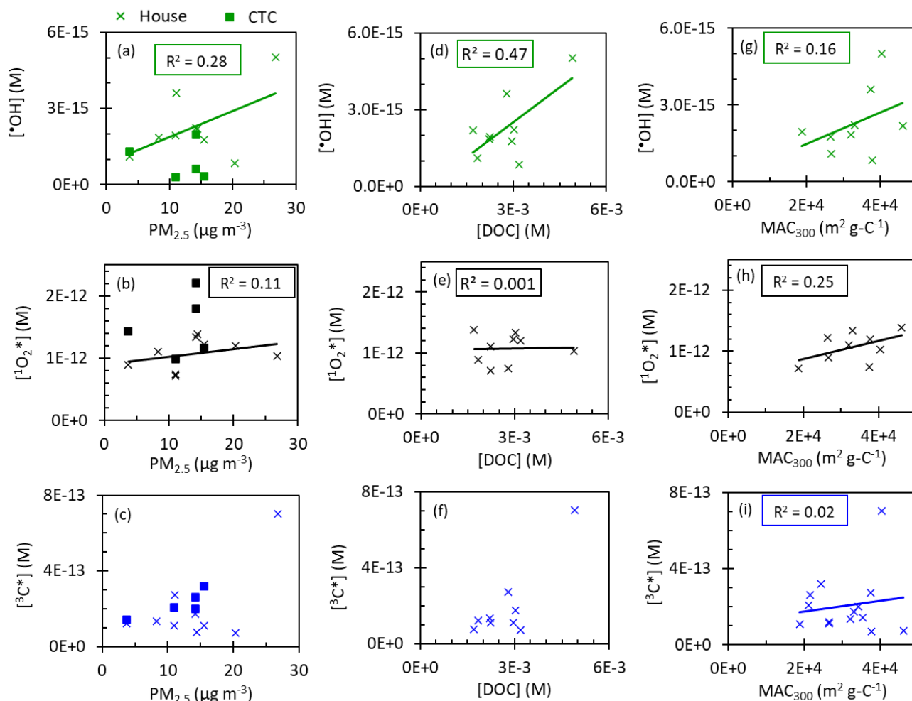
645 Figure S5. Correlations of \bullet\text{OH} , \text{}^1\text{O}_2^* , and \text{}^3\text{C}^* concentrations with \text{PM}_{2.5} , [\text{DOC}]_{\text{PME}} , and \text{MAC}_{300} . (a) – (c) all depict House (marked with 'x') and CTC site samples (marked with filled squares), while (d) – (i) only show House site samples. The regressions were calculated using only the House site samples to control for site differences. [\text{DOC}]_{\text{PME}} at the House and CTC sites cannot be compared because the filters at the two sites collected different size bins, with the House site representing \text{PM}_{2.5} and the CTC site representing \text{PM}_{0.7} .
