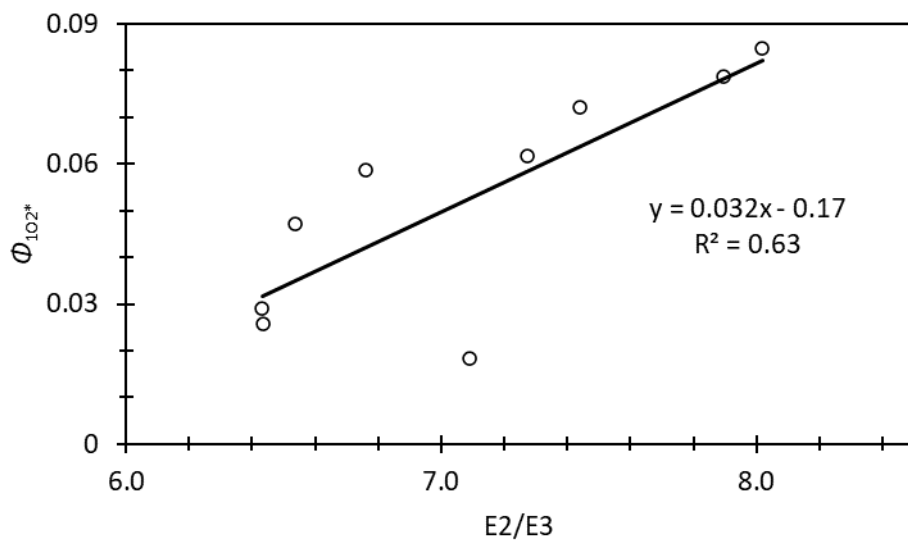
Figure S7. Relationship of \Phi_{102^*} and E2/E3 .
