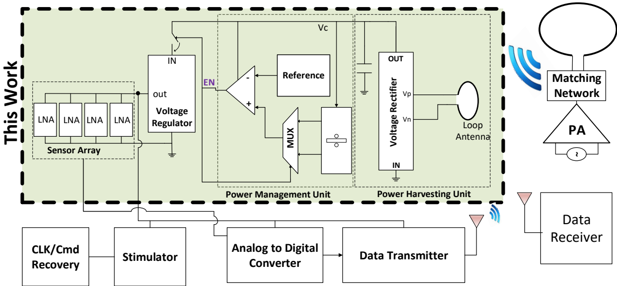
Figure 2.14. System architecture of the proposed power harvesting system.
