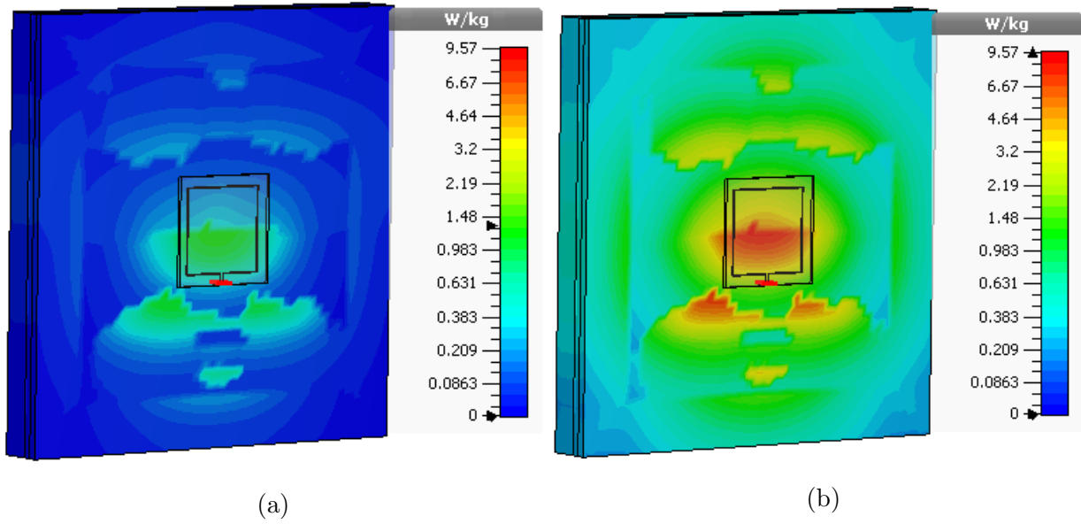
Figure 2.9. SAR distribution in multi-layer model of the human head averaged over 10 gram of tissue with a reference power of 1W input power. (a) 500 MHz (b) 2 GHz.
