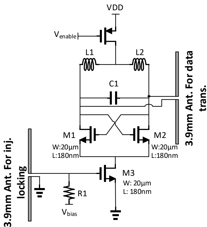
Figure 4.9. Circuit schematic of the injection-locked VCO.
