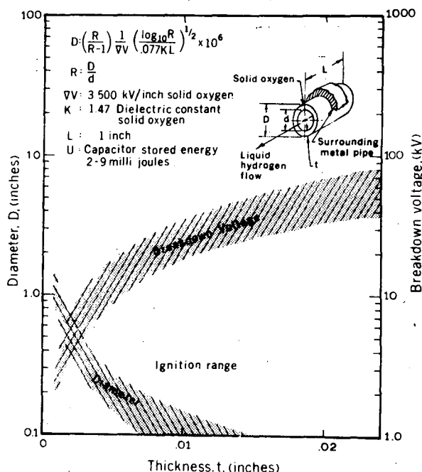
Fig. 3. Spark-induced potentially explosive range in a mixture of frozen oxygen and liquid hydrogen. Calculated potentially explosive range for various size frozen-oxygen cylinders capacitively charged by flowing liquid hydrogen. This figure shows the small volume of oxygen needed to store 2 to 9 mJ, which is a about 1000 times the 7 \mu J needed for ignition.
