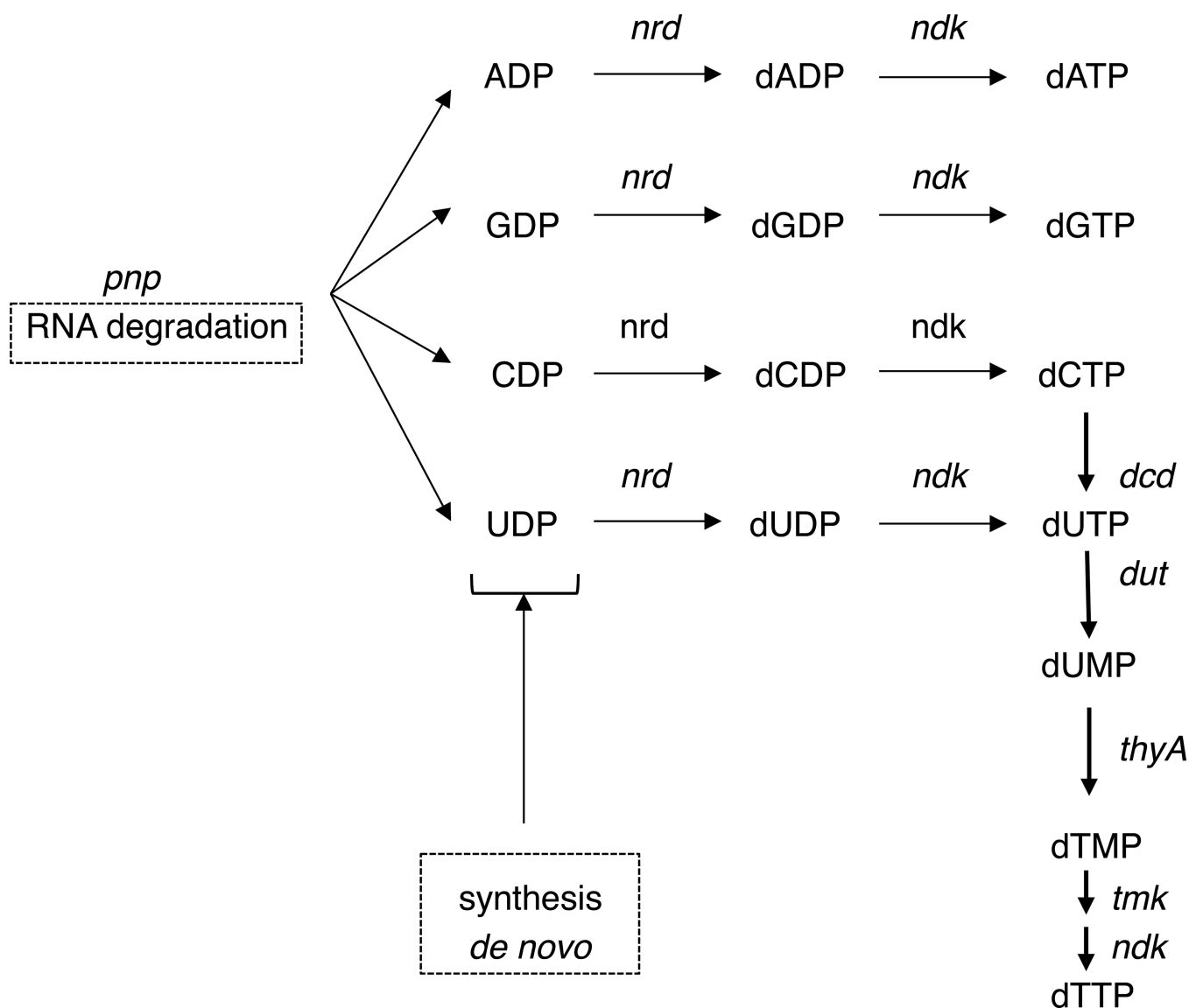
Fig. 1. Metabolic pathway for thymidine biosynthesis in Escherichia coli .
