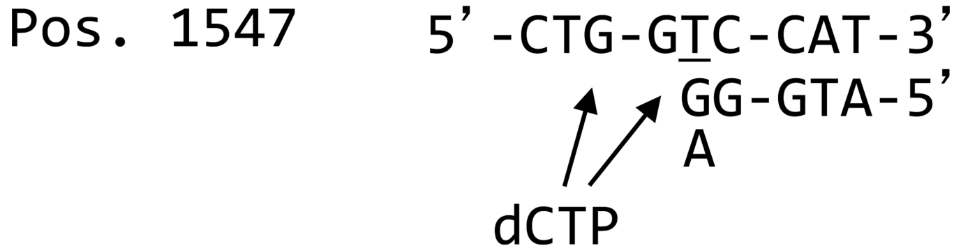
The next-nucleotide effect. Diagram showing how elevated dCTP levels affect the rpoB mutation rate at hotspot positions 1534 and 1547. In each case, the A·T→G·C transition responsible for the Rif r phenotype is represented as mediated by a T·G polymerase error. (The shown templates represent rpoB coding and non-coding strands, respectively, for 1534 and 1547). During the misinsertion event, the incorrect G is competing with the correct A. Following the misinsertion, competition ensues between the extension of the mismatch by incorporation of the next nucleotide dCTP, which would fix the mutation, with the exonucleolytic removal of the G. High levels of dCTP will push the forward reaction and, are therefore predicted to be mutagenic. Note that for the hotspot at position 1547 two dCTP incorporations follow the mismatch, consistent with the exceptionally high mutation rate for this site in response to elevated dCTP.
