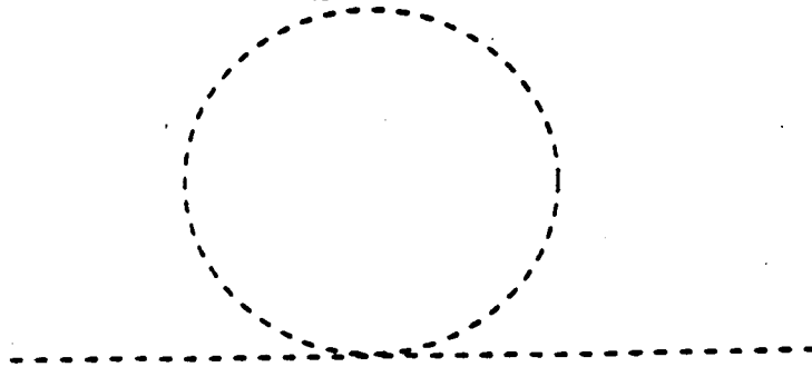
Figure 4.1: Quadratically divergent contribution to Higgs boson self-energy, as in eq. (4.1).
