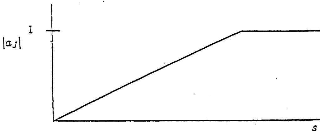
Figure 6.7: Extrapolated low energy theorem for strong W^+W^+ scattering, eq. (6.9).
