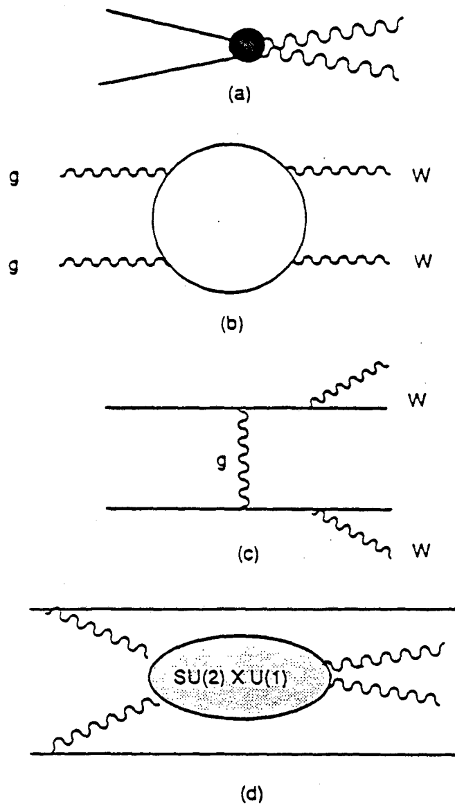
Figure 6.2: Backgrounds to H \rightarrow WW signal from (a) \bar{q}q \rightarrow WW , (b) gg \rightarrow WW via \bar{Q}Q loops, (c) gluon exchange, and (d) higher order O(g^4) electroweak interactions including WW fusion as shown.
