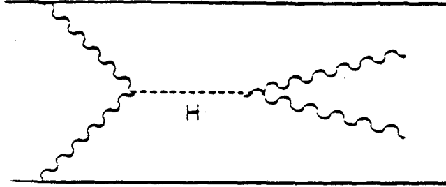
Figure 6.4: Higgs boson production via WW fusion and decay to WW .
