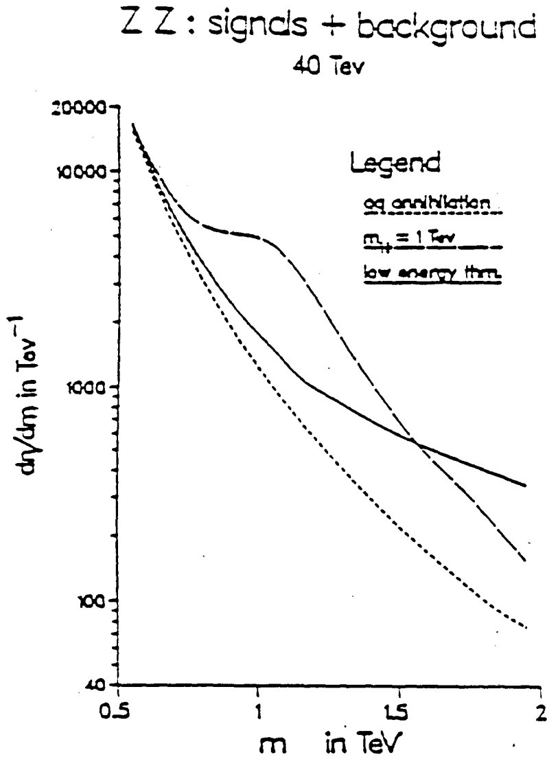
Figure 6.6: Yields defined as in figure 6.5 for a 40 TeV pp collider. The short dashed line is the \bar{q}q \rightarrow ZZ background while the long dashed line is the sum of the background and the H \rightarrow ZZ signal. The solid line represents the sum of signal plus background for an extrapolation of the low energy theorem as discussed in Section 6.2 (from ref. 3).
