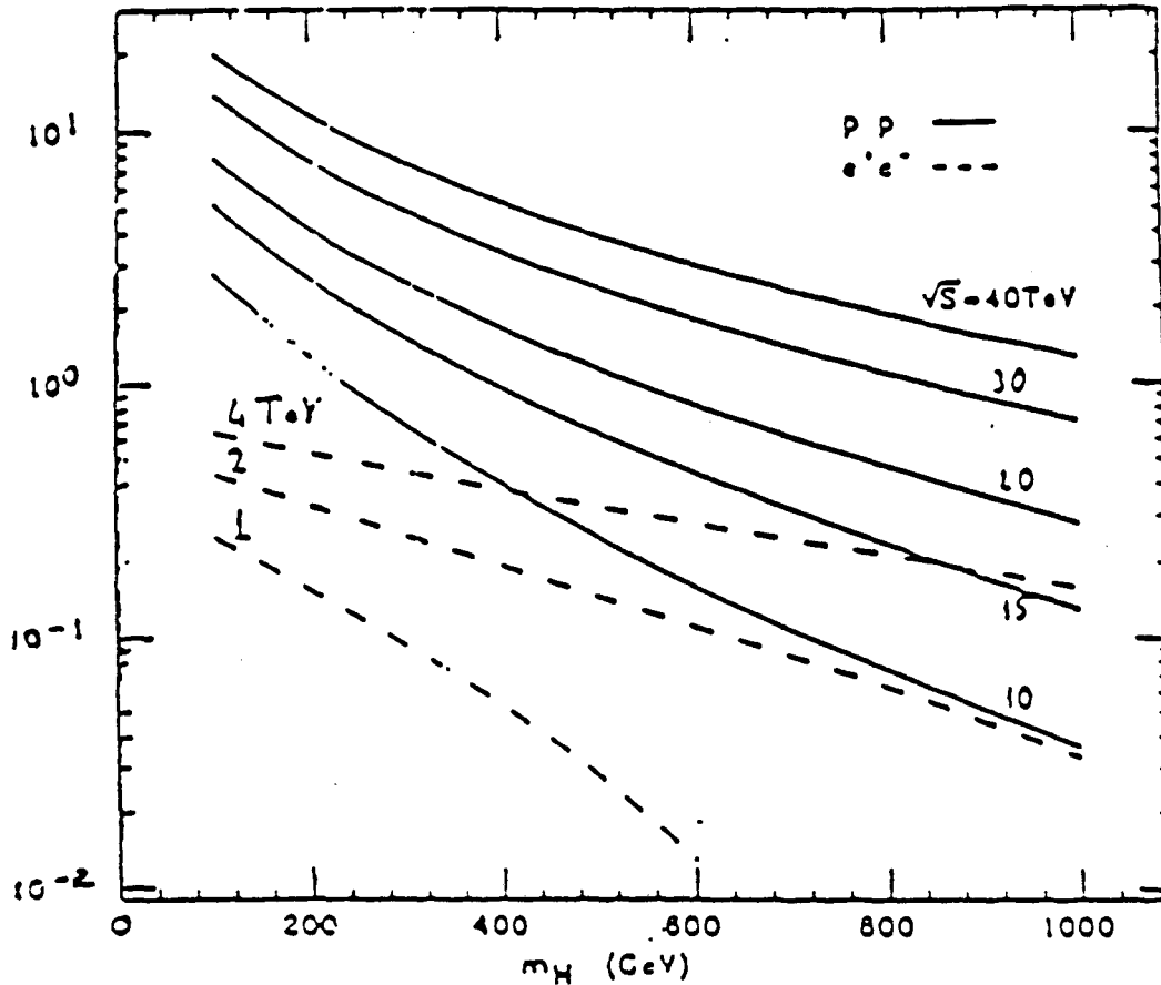
Figure 6.3: Higgs boson production cross sections in picobarns at e^+e^- and pp colliders with center of mass energies indicated (from ref. 42a).
