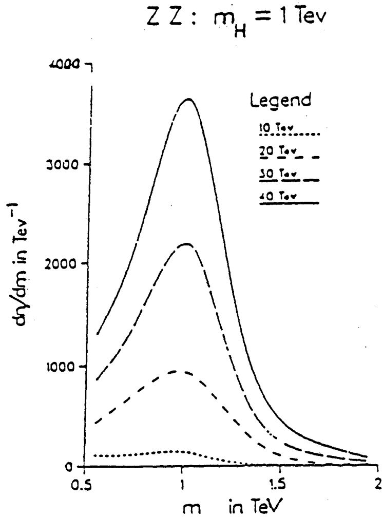
Figure 6.5: Yield \frac{dn}{dm_{ZZ}} in \text{TeV}^{-1} for H \rightarrow ZZ at 10, 20, 30, and 40 TeV pp colliders, in events per 10^4 \text{pb}^{-1} with |y_Z| < 1.5 (from ref. 3).
