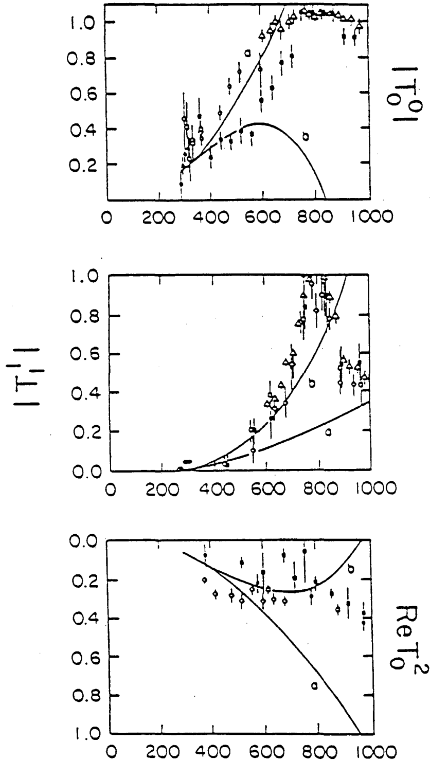
Figure 6.8: Data for \pi\pi partial wave amplitudes compared with extrapolated low energy theorems (e.g., eq. (6.9)) for the three channels I; J = (0,0), (1,1), (2,0) . The curves labeled a correspond to the naive extrapolation as in eq. (6.9) and figure 6.6. The figures are from ref. 53.
