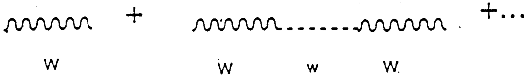
Figure 2.1: Geometric series for the W propagator corresponding to eq. (2.35).
