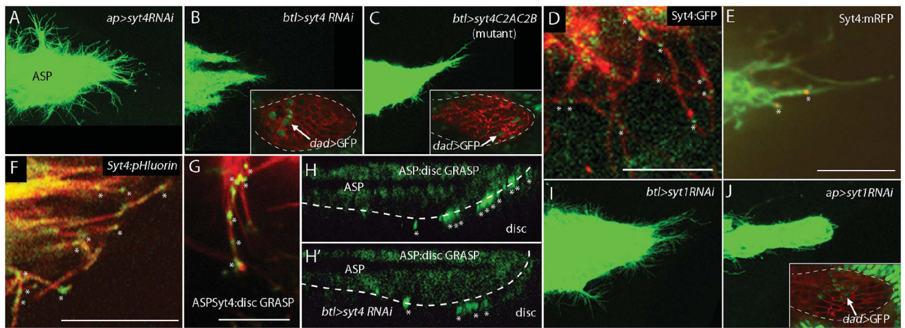
Fig. 3. Cytoneme-mediated transport requires Syt4.
