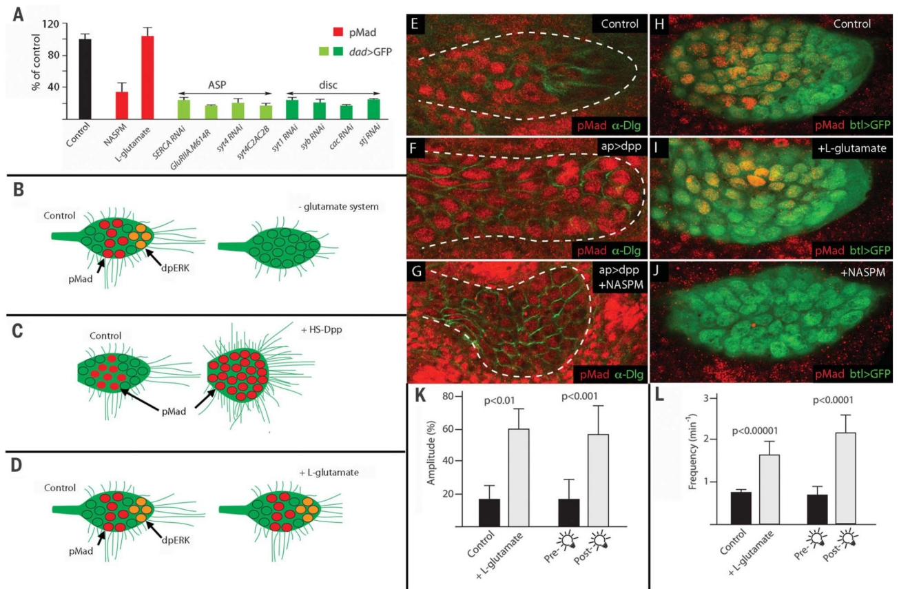
Fig. 5. Dependence of Dpp signaling on glutamate and synaptic proteins.
