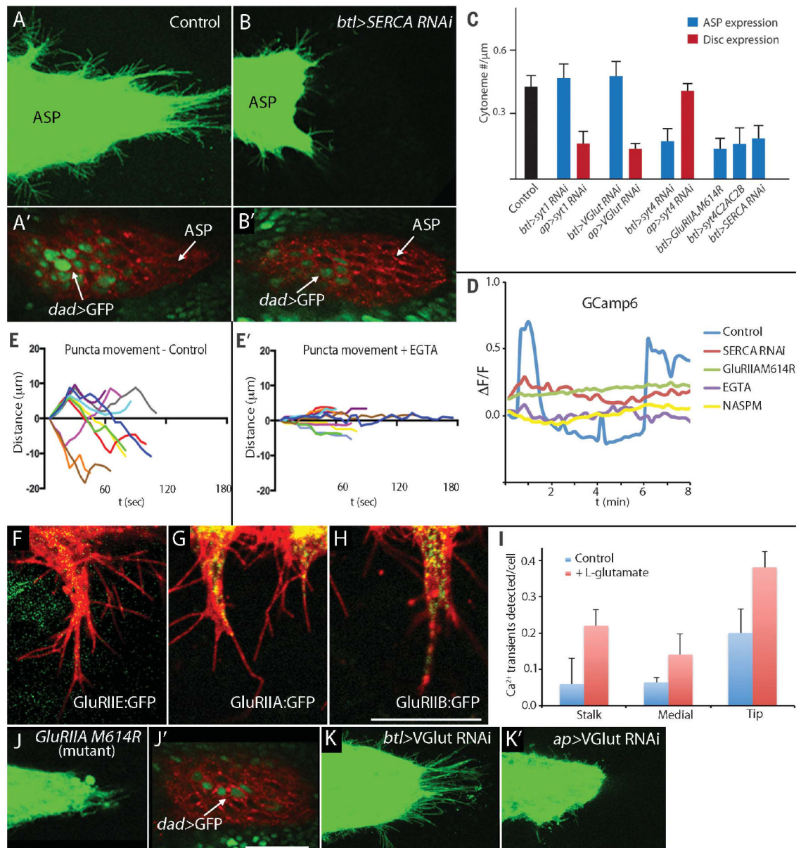
Fig. 2. Cytome-mediated transport requires SERCA and GluR.
