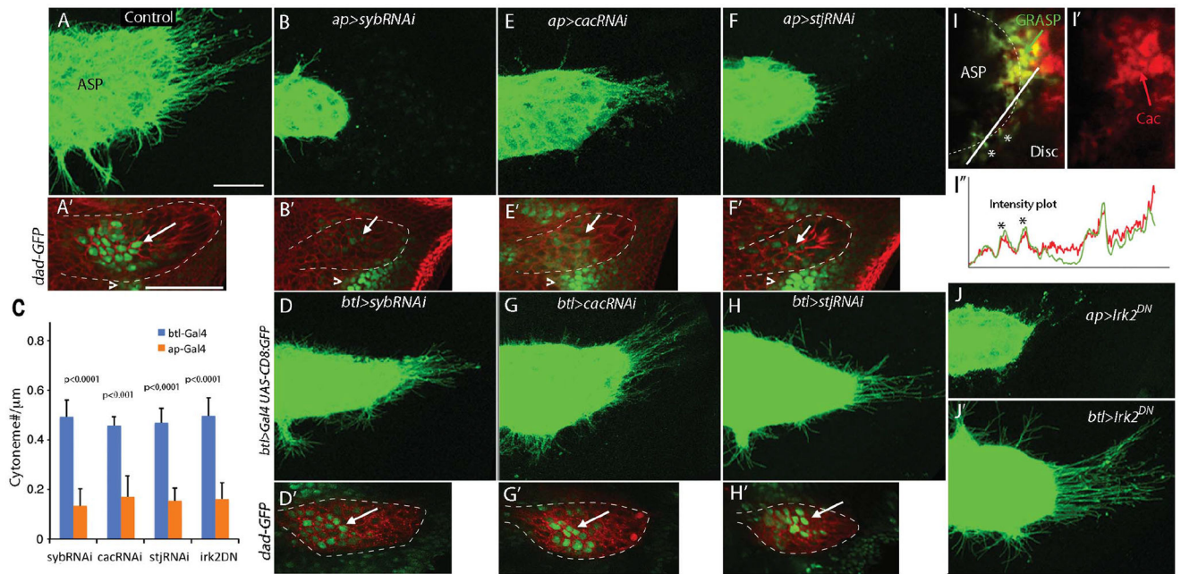
Fig. 4. The ASP depends on the VGCC and Syb SNARE in the wing disc.
