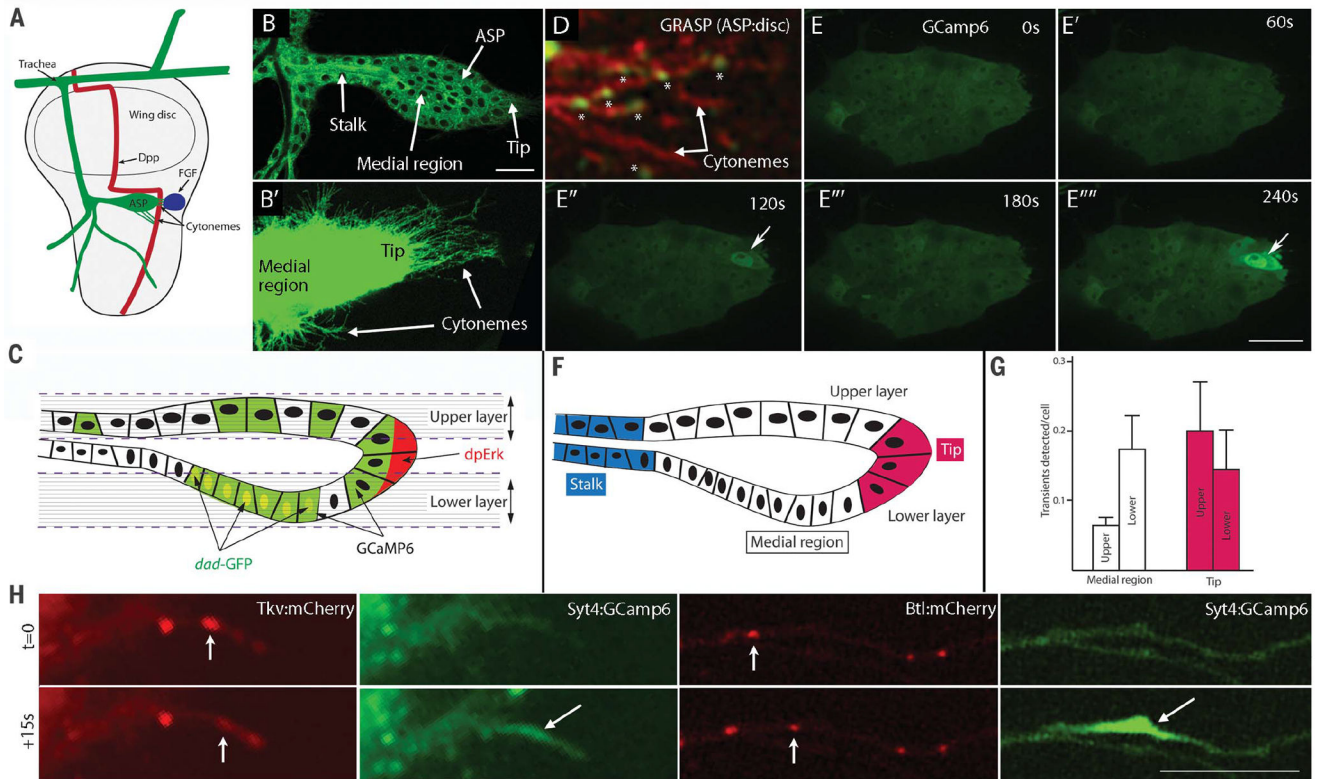
Fig. 1. Calcium transients in the ASP and ASP cytonemes.
