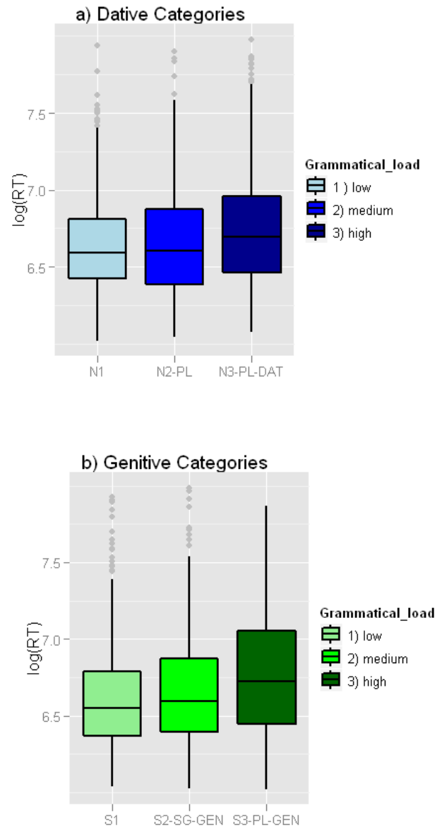
Figure 1: Boxplots for log(RTs), inflectional categories (x-axes), and grammatical load indicated by color.
