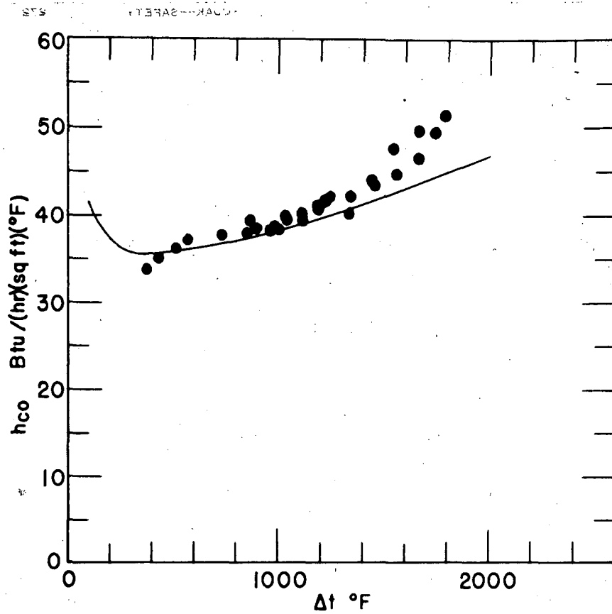
FILM BOILING OF ETHYL ALCOHOL FROM 0.352" CARBON TUBE FIG. 10
