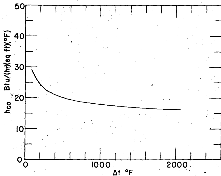
FILM BOILING OF MERCURY FROM 0.352" CARBON TUBE
