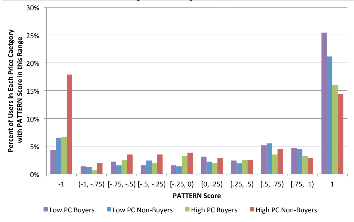
Figure 3. Frequency Distribution of PATTERN for Buyers and Non-Buyers in Low and High Price Categories (PC)
