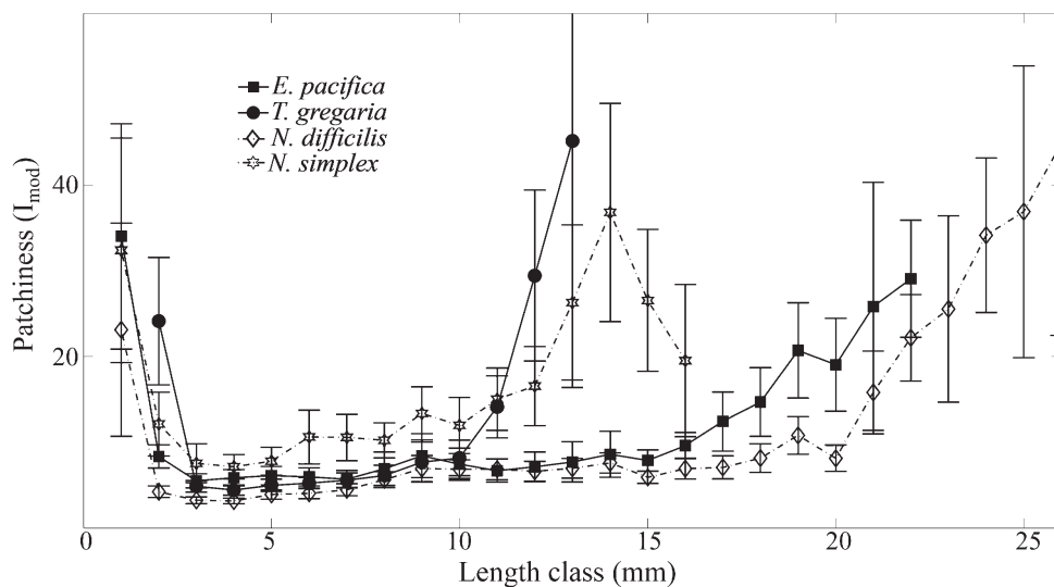
Fig. 8. Patchiness ( I_{\text{mod}} , mean \pm 95 C.I.) vs. total length for euphausiid species displaying two reproductive modes: broadcast spawners (black; E. pacifica and T. gregaria ) and egg brooders (gray; N. difficilis and N. simplex ).
