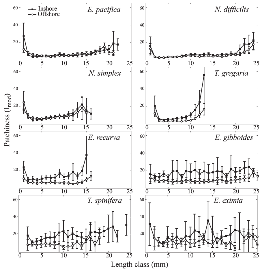
Fig. 7. Contrast between the inshore (black) and offshore (gray) regions in patchiness ( I_{\text{mod}} ) vs. total length for the eight euphausiid species (mean \pm 95 C.I.).
