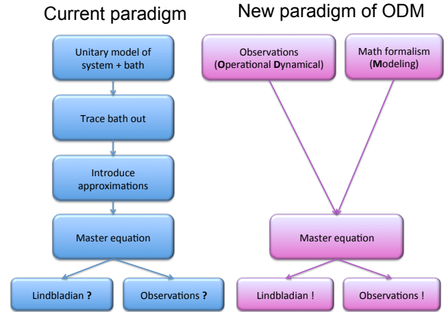
Figure 1: Currently paradigm for deriving master equations governing open system dynamics vs proposed novel approach of Operational Dynamic Modeling (ODM).
