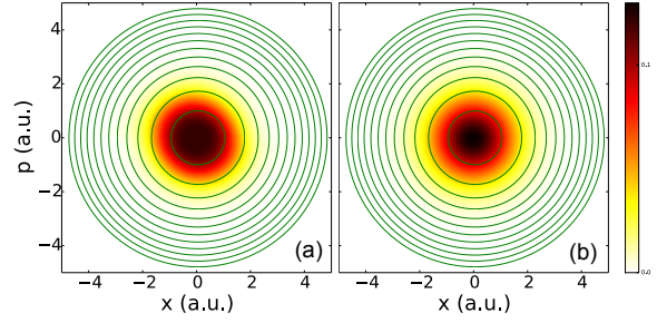
Figure 3: (a) The final Wigner function for the harmonic oscillator evolving according to the model (1) governing the Ohmic dissipation [with eq (20), \gamma = 0.07 a.u., L = 3 a.u., and \mathfrak{D} = 0.0143 a.u.]. The circular solid lines depict the level set of the Hamiltonian H = (p^2 + x^2)/2 a.u. The initial Wigner function is shown in figure 2(a). Note that the steady state approaches the thermal Boltzmann state with kT = 1.166 a.u. depicted in (b).
