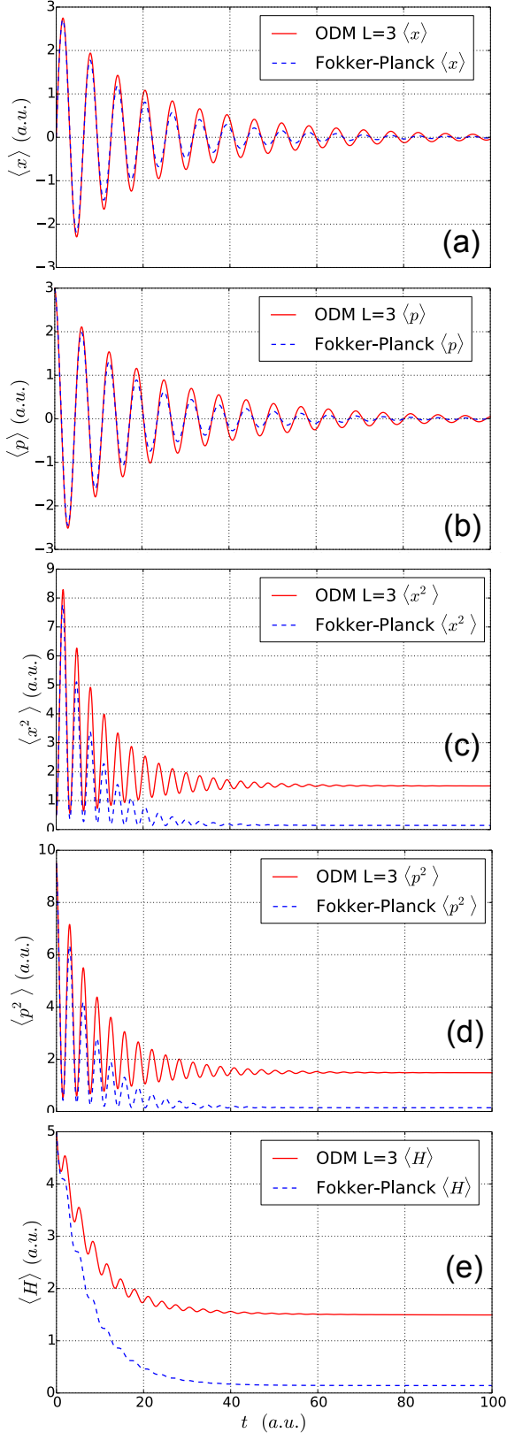
Figure 5: Quantum (solid red lines) [eq (1)] vs classical (dashed blue lines) [eq (9)] dissipative dynamic of a harmonic oscillator. Parameters for both systems are identical (parameters are specified in figure 3.) Time-evolution of the first [(a), (b)] and second [(c), (d)] order moments. (e) The total energy variation.
