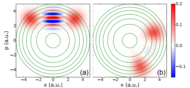
Figure 4: (a) The Wigner function of the Schrödinger cat state at time t = 0 . (b) The Wigner function at later time t = 2 a.u. after evolving according to the model (1) governing the Ohmic dissipation (system's parameters are defined in figure 3). As time progresses, the Wigner function's negativity vanishes and the state approaches the Boltzmann equilibrium shown in figure 3(b).
