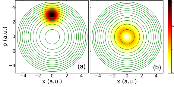
Figure 2: The initial (a) and final (b) Wigner functions for the harmonic oscillator evolving according to the model (1) governing the Ohmic dissipation [with eq (20)], \gamma = 0.07 a.u., L = 3 a.u., and \mathfrak{D} = 0 . The circular solid lines depict the level set of the Hamiltonian H = (p^2 + x^2)/2 a.u. (a) The Wigner function of the ground state displaced along the momentum axis. The reached steady state (b) is not a Gaussian distribution.
