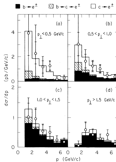
FIG. 1. Prompt-electron momentum spectra in four regions of transverse momentum p_\perp (GeV/c): (a) p_\perp < 0.5 , (b) 0.5 < p_\perp < 1.0 , (c) 1.0 < p_\perp < 1.5 , and (d) p_\perp > 1.5 . Two sets of error bars are shown for each data point. The smaller ones are statistical only. The larger ones are the statistical and systematic errors added in quadrature. The highest momentum bin includes all momenta \geq 6 GeV/c. The histograms show the results of the fit. The three contributions shown are (i) b primary (solid), (ii) c secondary (diagonally hatched), and (iii) c primary (unshaded).
