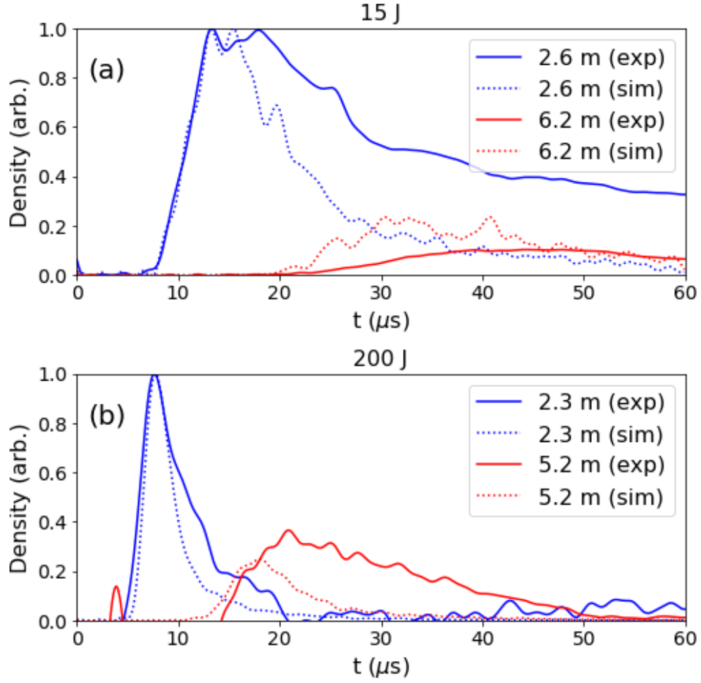
Figure 4.9: A comparison between two synthetic Langmuir traces created using results from the Monte-Carlo model and two experimental Langmuir ion saturation measurements recorded using the 15 J laser (a) and the 200 J laser (b). Each set of traces is normalized by the peak values of the probe closest to the target.
