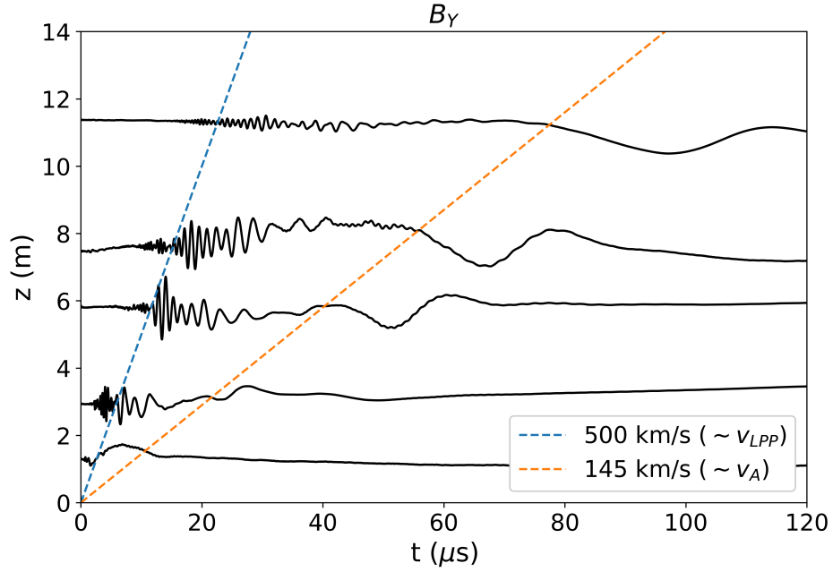
Figure 5.2: Measurements from an array of magnetic flux probes show a packet of waves propagating away from the laser target at a speed comparable to the super-Alfvénic LPP. A shear Alfvén wave follows, propagating at the Alfvén velocity.
