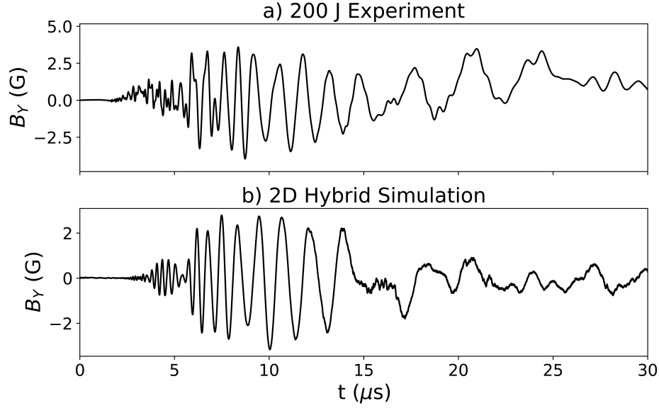
Figure 5.18: a) A measurement of B_Y from a magnetic flux probe 7.5 m from the target in the 200 J experiment. b) B_Y recorded by a corresponding virtual magnetic flux probe in the 2D hybrid simulation of the experiment. Simulation results provided by Martin Weidl.
