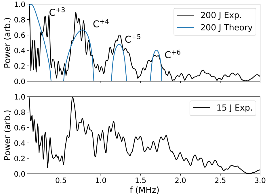
Figure 5.7: Fourier spectra of the B_Y signals shown in Fig. 5.1 show waves over a range of frequencies in both experiments. Predicted growth rates from linear theory (overplotted) show that these measurements are consistent with excitation of the RHI by various carbon charge states.
