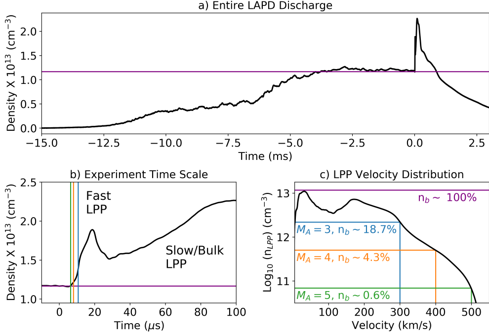
Figure 4.3: A microwave interferometer measurement over the entire duration of the LAPD discharge (a) shows that the LPP density is approximately equal to the LAPD \text{LaB}_6 density and dissipates slowly over \sim 1 ms. Looking more closely (b), the LPP is divided into a lower density burst of fast ions followed by a higher-density mass of slow ions (the “bulk”). An approximate velocity distribution calculated from these measurements (c) shows that the fastest LPP ions represent only a small fraction of the background density.
