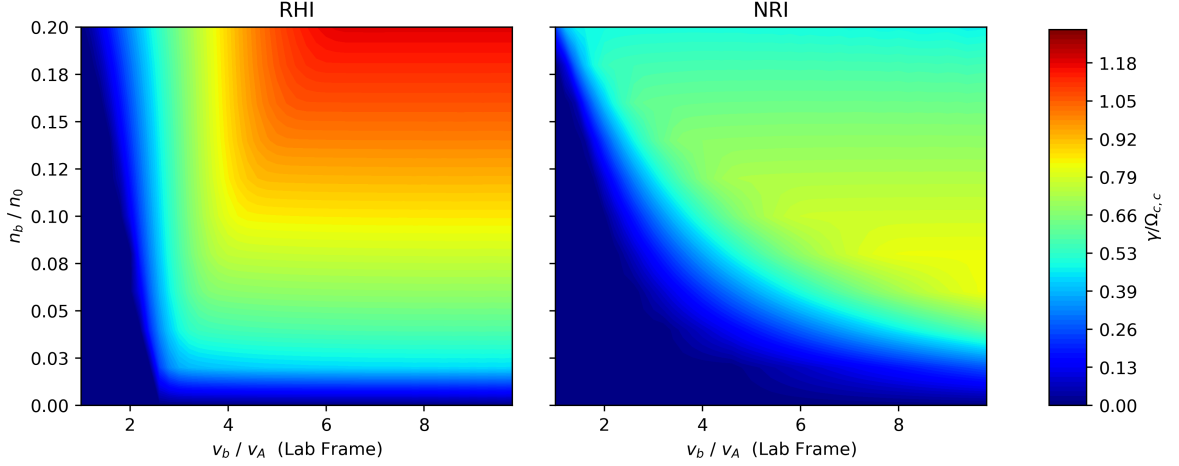
Figure 2.5: Growth rates for the RHI and NRI as a function of beam ion velocity and density. These growth rates are calculated for C^{+4} beam ions and He^{+1} core ions.
