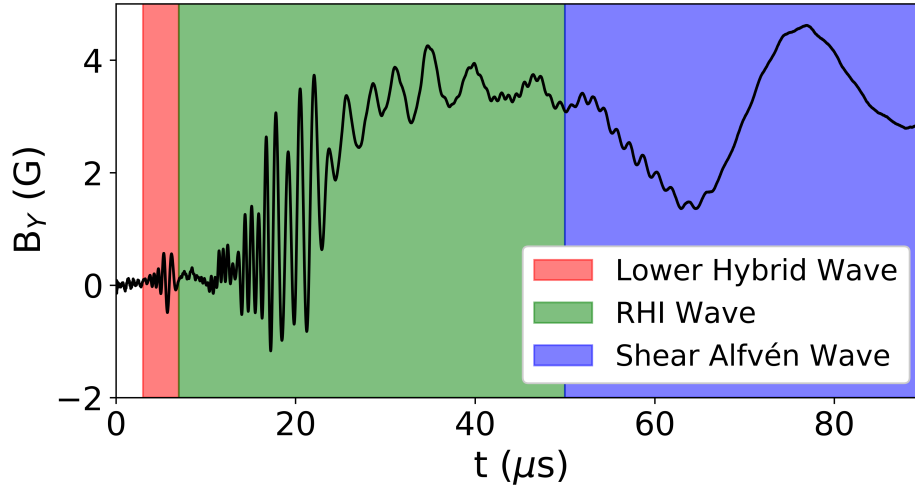
Figure 5.3: Three separable wave features are observed in the experiments: the lower hybrid wave, the RHI waves, and the shear Alfvén wave. These features travel through the LAPD with group velocities of approximately 1000 km/s, 400 km/s, and 150 km/s respectively.
