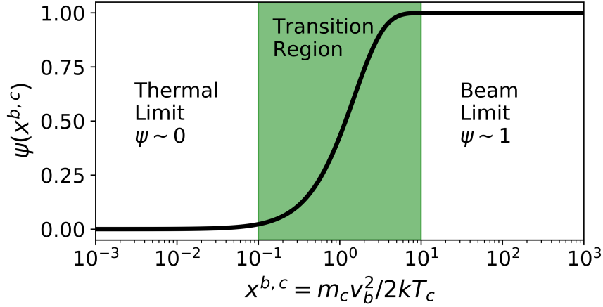
Figure 4.5: The Coulomb collision frequencies depend on the \psi function (Eq. 4.4) whose argument is the ratio between the plasma's directed (beam) and thermal kinetic energies (Eq. 4.2). For a fast beam \psi = 1 while for a thermal plasma \psi = 0 . Simplified expressions for the collision frequencies can be written in either limit. In the intermediary range where the ratio between the beam and thermal energies is between 0.1 and 10, \psi must be calculated explicitly.
