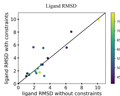
Figure 5. Analysis of the ligand rmsd of the 17 enzymes from the benchmark when docking was performed on the lowest five models with and without the incorporation of the enzymatic constraints. The rmsd was determined by the heavy atoms of the ligand and comparing the target crystal structure ligand to the docked ligand of the models. Each point represents the average rmsd of the lowest five models, and the color of each point in the graphs represents the percent identity of the top template used for modeling.
