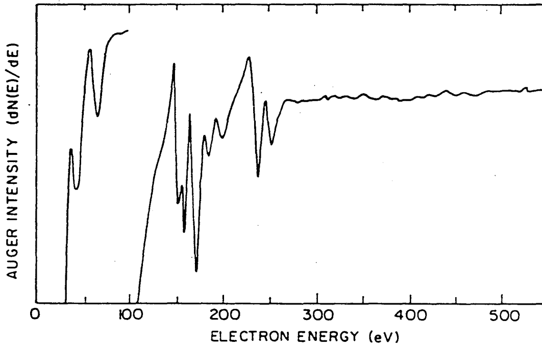
Figure 3.2. The Auger process and the resulting Auger spectrum of a Pt surface.
