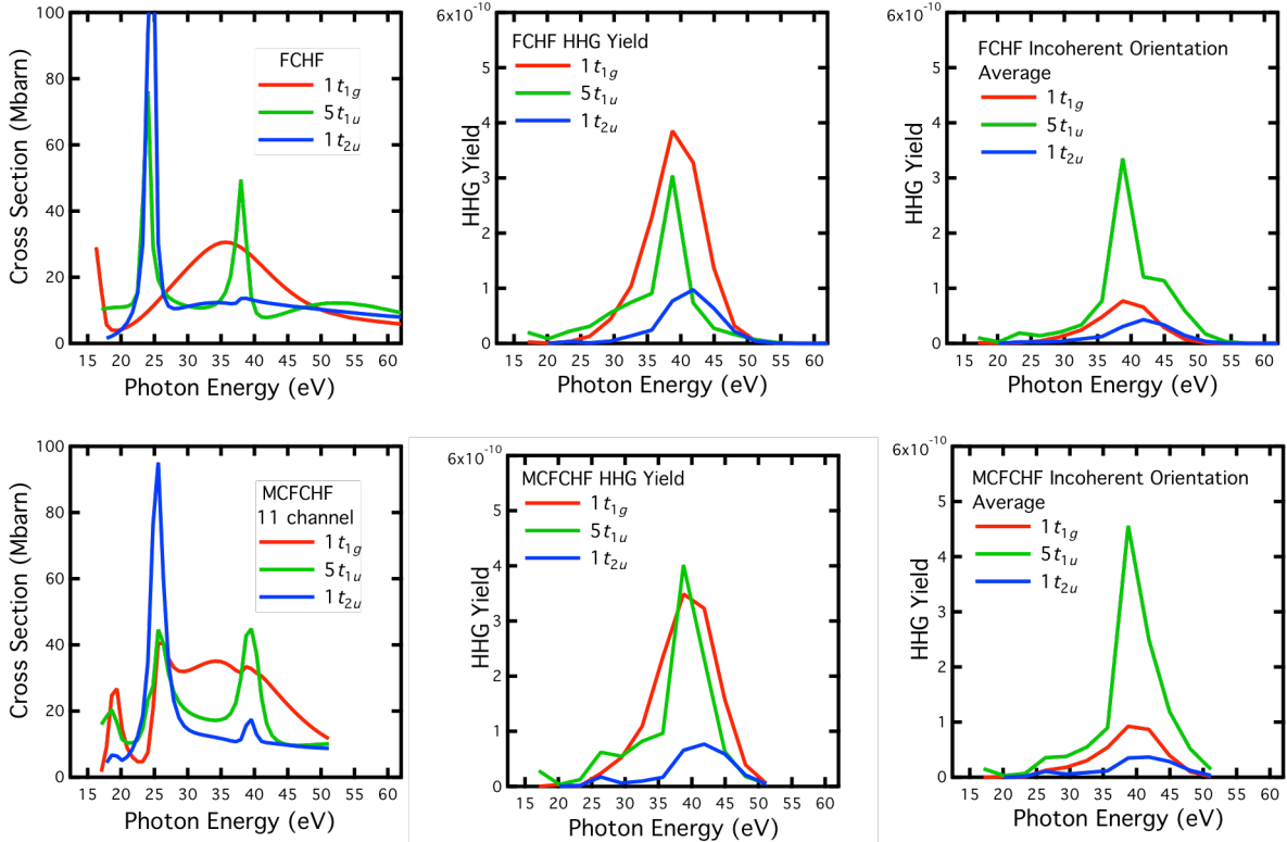
Figure 4. Photoionization cross sections and QRS HHG spectra of SF 6 for the outer three valence orbitals, 1t_{1g} (HOMO), 5t_{1u} (HOMO-1), and 1t_{2u} (HOMO-2). Left column is the computed photoionization cross sections. Center column is the QRS HHG spectra from the different channel terms in Eq. (3), which has a coherent orientation average. Right column is the approximate separate-channel HHG spectra obtained from the incoherent orientation average given in Eq. (4). The top row contains the results for the single-channel FCHF calculations and the bottom row has the corresponding data from the coupled channel MCFCHF calculations.
