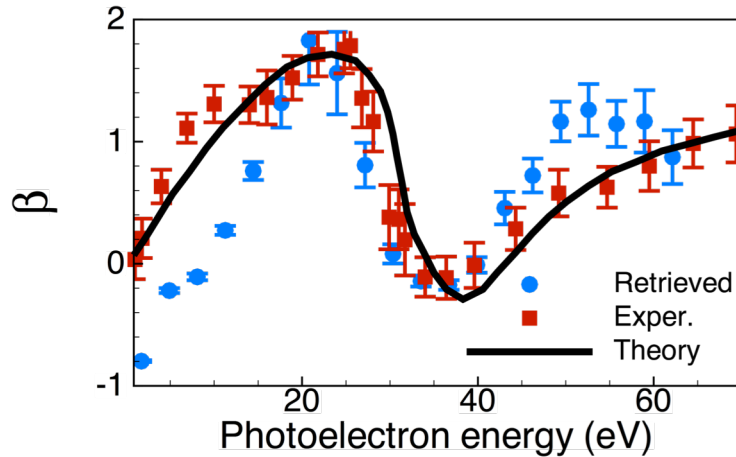
Figure 2. Energy dependence of the Ar 3p subshell photoelectron asymmetry parameter \beta(E) . Solid line: RPAE theoretical results 1 ; red squares: experimental photoionization results 2 ; blue circles: present results retrieved from HHG spectra.
