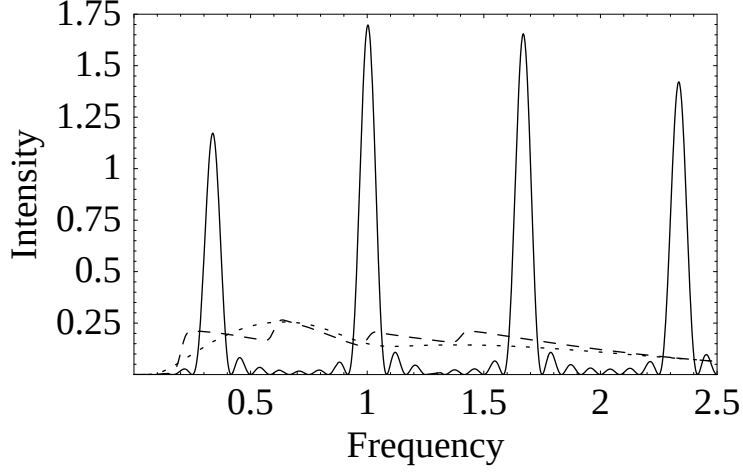
FIGURE 1. Normalized spectrum d^2 I(0)/d\omega d\Omega (arbitrary units) versus \omega/2\gamma_{z0}^2\omega_\beta for the first four harmonics ( n = 1, 2, 3 , and 4 ) with N_\beta = 4 . The solid curve shows the radiation from a single electron with a_\beta = \gamma_{z0}k_\beta r_\beta = 4 . The dashed (dotted) curve shows the spectrum integrated over a flat-top (Gaussian) distribution of betatron amplitudes r_\beta with a_{\beta,rms} = \gamma_{z0}k_\beta r_{\beta,rms} = 4 .
