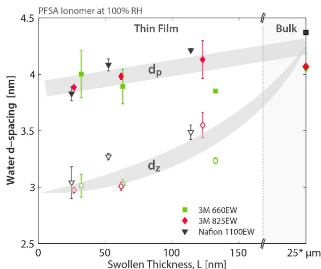
Figure 10 Hydrophilic domain spacing of vapor-saturated PFSA ionomers across the lengthscales, i.e. from bulk to thin films, plotted in the plane and thickness direction as a function of film thickness. The values for the bulk membranes are shown at 25 micron for ease of plotting.
