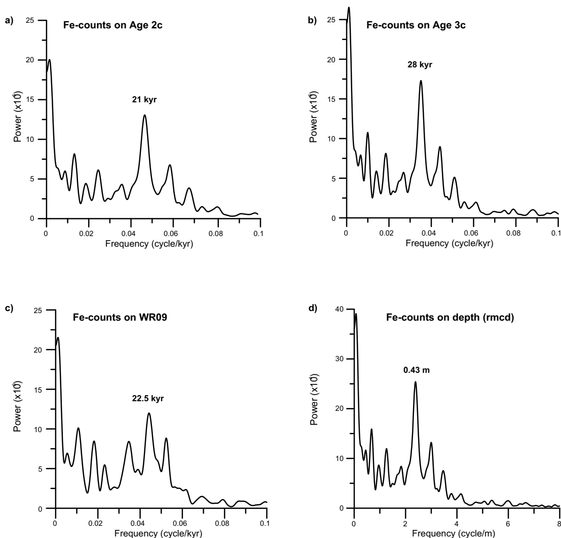
Fig. 7. Power spectra of the Fe-record in the problematic interval from of Site 1258 using a) 2-cycle age model: b) 3- cycle age model and c) the initial age model by Westerhold and Röhl (2009) d) depth scale (rmcd).
