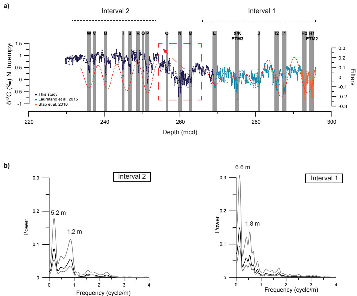
Fig. 2. a) Benthic N. truempyi \delta^{13}C record from Site 1263 plotted versus depth (mcd). Highlighted intervals represent the position of the early Eocene hyperthermal events and subsequent excursions in the carbon isotope data, labelled alphabetically extending the nomenclature initiated by Cramer et al. (2003). Dashed lines represent bandpass filters applied to the lower and upper intervals. The red box indicates the “problematic interval” characterized by a \sim 1\text{‰} positive shift in the carbon values. b) Power spectra of the two intervals selected for the construction of the age models.
