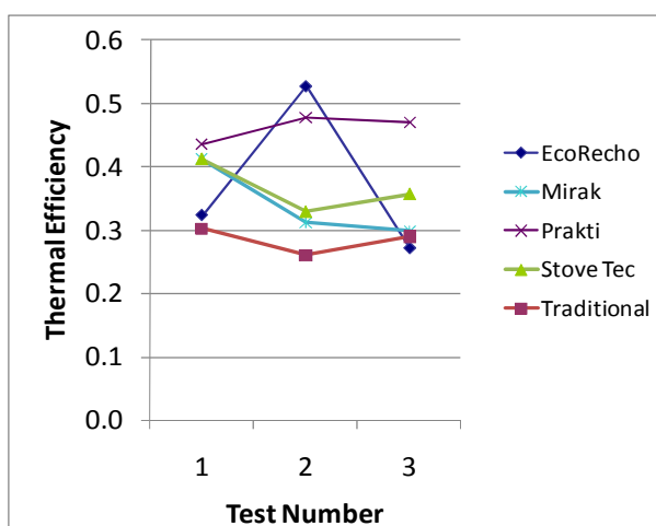
Fig. 6: Thermal Efficiency, Simmer Phase by Test.
