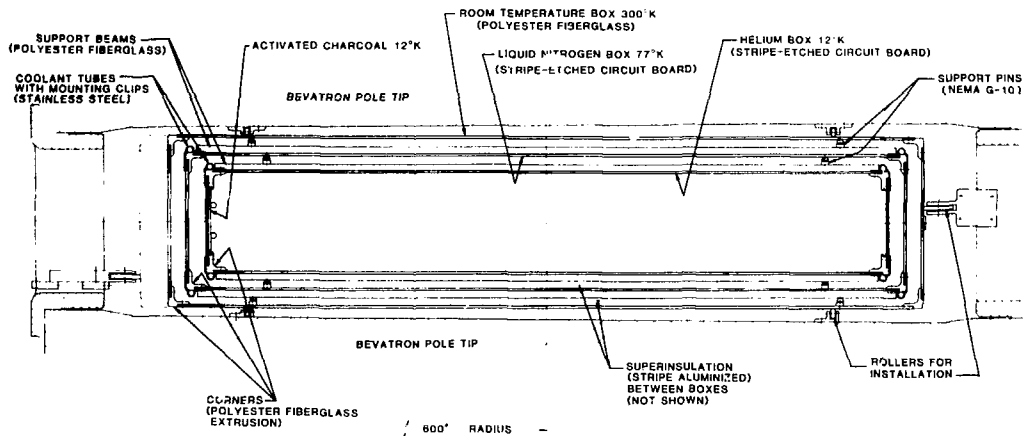
Fig. 2. Cross-section of quadrant liner between Bevatron poletips.
