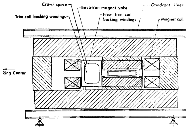
Fig. 1. Bevatron quadrant cross-section.
