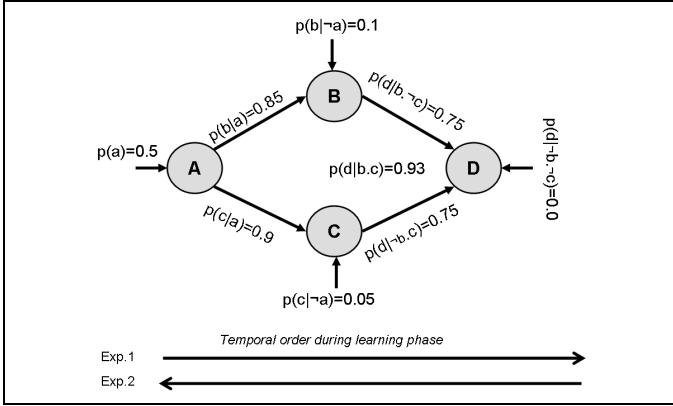
Figure 1: A parameterized causal model. Arrows indicate causal relations between variables; conditional probabilities encode the strength of these relations. All parameters were set except p(d|b,c) which is computed by a noisy-OR-gate.
