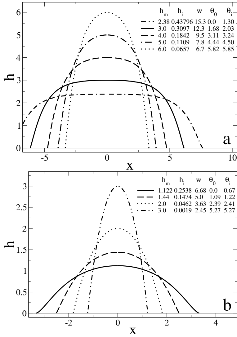
Fig. 5. Different drop profiles for Bi = 0.5 , Bo = 1.0 and fixed volume (a) L = 30 , Ma = 3.5 , (b) L = 5 , Ma = 1.5 . The maximum thickness h_{max} , the thickness h_i at h_{xx} = 0 and the width w of the drop are listed, as are the contact angles \theta_0 = h_x(0) and \theta_i = h_x(h_i) .
