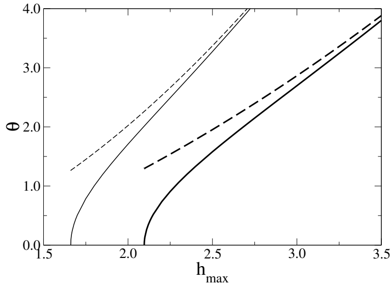
Fig. 6. The microscopic ( \theta_0 , solid lines) and mesoscopic ( \theta_i , dashed lines) contact angles as a function of the maximum film thickness when \text{Bi} = 0.5 , \text{Bo} = 1.0 , \text{Ma} = 3.5 and fixed volume L = 5 (thin lines) and L = 10 (thick lines).
