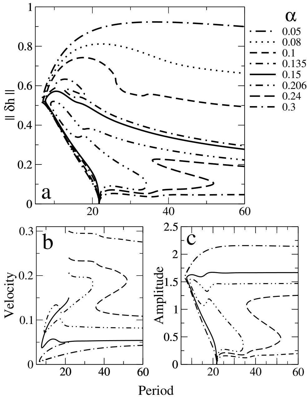
Fig. 8. Traveling wave solutions of Eq. (1) along the n = 1 primary branch as a function of L when Ma = 3.5 , Bi = 0.5 and Bo = 0.5 . (a) The L_2 norm of \delta h \equiv h(x) - 1 for different values of the inclination \alpha . (b) The corresponding drift velocity v . (c) The amplitude \Delta h \equiv h_{max} - h_{min} . The linestyles in (b) and (c) correspond to those used in (a). The saddle-node departs from its location at L \approx L^* once \alpha > 0.2 .
