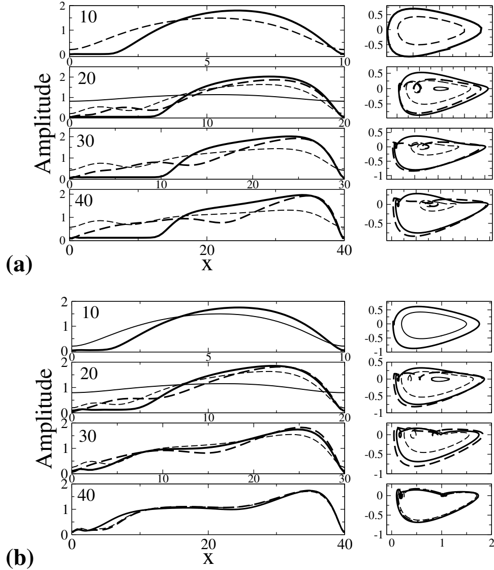
Fig. 14. Profiles of primary (solid lines) and secondary (dashed lines) n = 1 solutions for Ma = 3.5 , Bi = 0.5 , Bo = 0.5 and different periods L when (a) \alpha = 0.08 , (b) \alpha = 0.113 . Thick (thin) lines refer to upper (lower) parts of each branch as in Fig. 10. Note the asymmetry in the profiles and the development of an extended 'dry' spot as L increases. The solutions in (b) develop an undershoot just before the front of the drop; this undershoot manifests itself as a small spiral in the (h, h_x) phase portraits shown in the right set of panels. The secondary solutions along the dotted branch in Fig. 10 are not shown.
