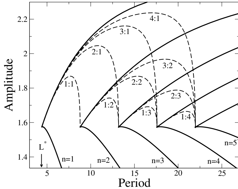
Fig. 4. The amplitude \Delta h \equiv h_{max} - h_{min} along single drop and multidrop branches with microscopic contact angle \theta_0 = 0 as a function of L when Ma = 3.5 , Bi = 0.5 and Bo = 1.0 (cf. Fig. 2a). The solid lines show the primary n = 1, \dots, 5 branches consisting of periodic nucleation solutions (lower part) and the periodic single drop solutions (upper part) obtained by replication of the n = 1 solution. The dashed lines show the different possible multidrop branches with maximal internal symmetry and no dry holes. Multidrop solutions with broken internal symmetry are present between these multidrop branches as described in the text. Every multidrop solution of this type in turn represents the starting point for i + j branches containing finite dry holes.
