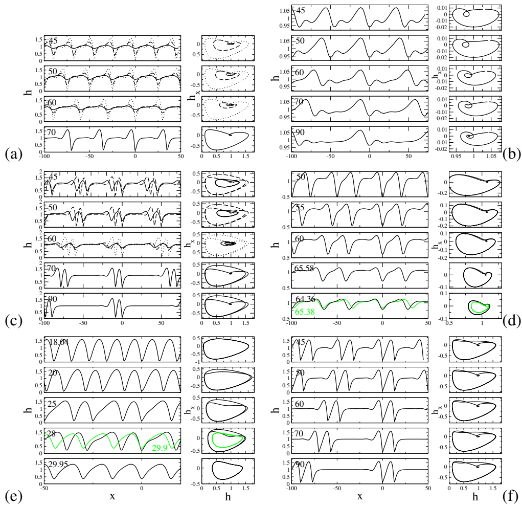
Fig. 17. Film thickness profiles along the n = 2 primary branch (panel a) and the n = 2 secondary branches (panels b-f) when Ma = 3.5 , Bi = 0.5 , Bo = 0.5 and \alpha = 0.2 for different periods as given in the legends. The respective branches are indicated in Fig. 16(b) by the corresponding letter. In cases where a given value of L cuts a branch in several locations the solid line refers to the upper solution, dashed to the middle and the dotted to the lowest.
