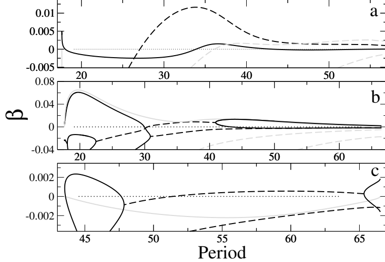
Fig. 20. The real parts of the largest eigenvalues \beta along the n = 2 primary branch when \text{Ma} = 3.5 , \text{Bi} = 0.5 , \text{Bo} = 0.5 and \alpha = 0.2 . Panels (a-c) refer to the upper, middle and lower parts of the branch. The solid (dashed) lines indicate real (complex) eigenvalues. The gray (black) lines refer to symmetry-preserving (-breaking) perturbations. The figure reveals intervals of stability on both the lower and upper parts. The part between the two saddle-nodes (Fig. 16b) is unstable everywhere.
