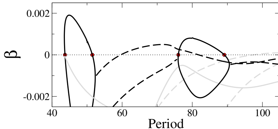
Fig. 21. The real parts of the largest eigenvalues \beta along the n = 2 primary branch when Ma = 3.5 , Bi = 0.5 , Bo = 0.5 and \alpha = 0.8 (Fig. 16d) showing intervals of stability in 51 < L < 60 and 89 < L < 97 . The solid (dashed) lines indicate real (complex) eigenvalues. The gray (black) lines refer to symmetry-preserving (-breaking) perturbations.
