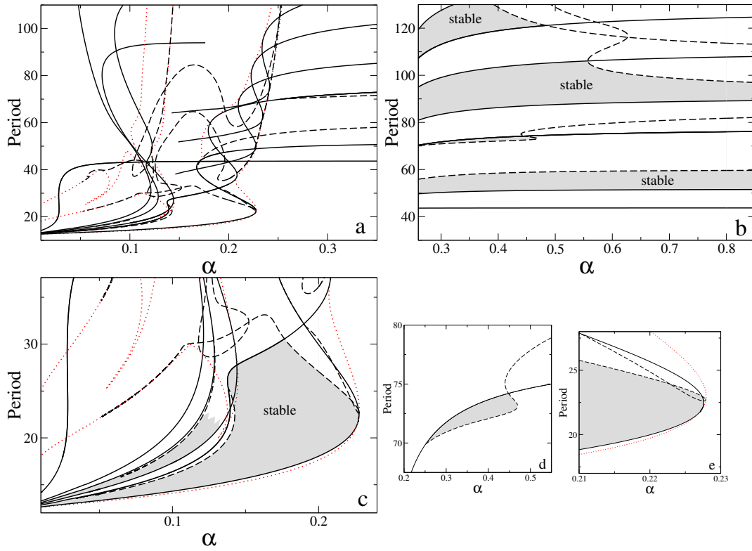
Fig. 22. Loci of bifurcation points on the n = 2 primary branch as a function of the inclination \alpha for Ma = 3.5 , Bo = 0.5 and Bi = 0.5 . The solid (dashed) lines represent steady state (Hopf) bifurcations. The dotted lines stand for the saddle-nodes already shown in Fig. 9 but scaled for the n = 2 branch. Panel (a) shows the transition between the small and large \alpha regimes, while (b) and (c) show the large and small \alpha regime, respectively. Regions where the primary n = 2 branch is linearly stable are shaded gray. Only the first two bands of stable solutions are indicated. The shading of the second band is discontinued near the necking bifurcation (see text), which reorders the branches. The enlargement (d) shows a region where a Takens-Bogdanov bifurcation is present while (e) zooms in on the disappearance of an isola.
