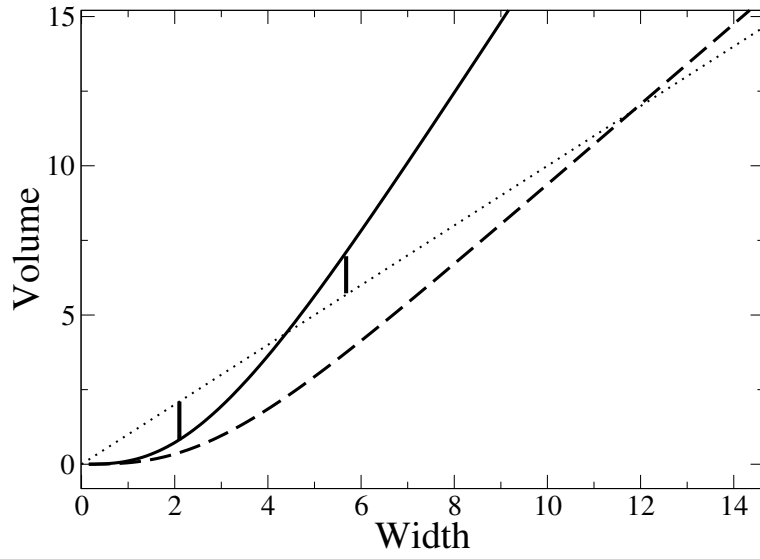
Fig. 3. The drop volume L as a function of its width w for \text{Ma} = 3.5 (solid line) and \text{Ma} = 1.5 (dashed line) along the thick dashed line in Fig. 2. The dotted line indicates the relation L = w . The intersections define the points L^* . Dry spots are present when L > w . The vertical lines indicate the construction of a two-drop solution corresponding to the maximum along the 1:1 branch in Fig. 4 (see text).
