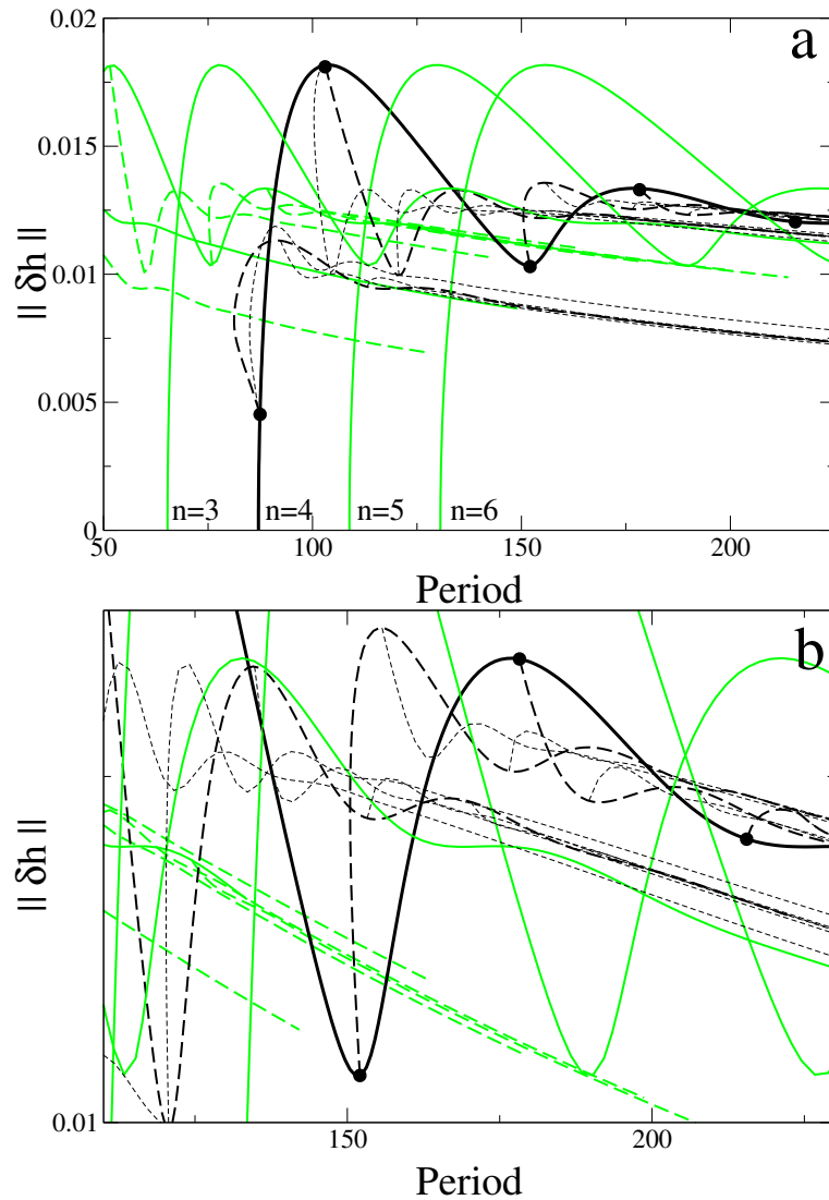
Fig. 23. The n = 4 primary (solid black line), secondary (dashed black line) and tertiary (dotted black line) branches for Ma = 3.5 , Bi = 0.5 , Bo = 0.5 and \alpha = 0.8 . Solid gray lines show the corresponding n \neq 4 primary branches, while dashed gray lines show secondary n = 2 branches. Panel (b) shows a detail of (a). Secondary bifurcations are indicated by solid black dots.
