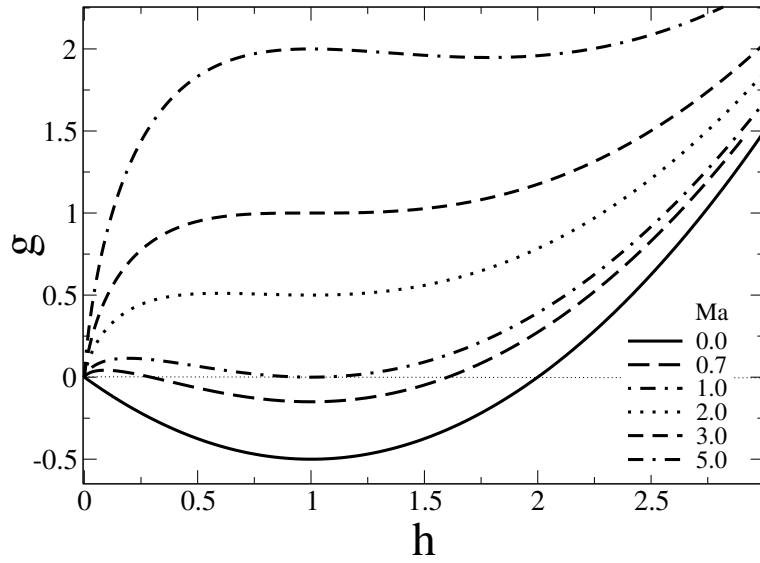
Fig. 1. The energy g(h) \equiv f(h) - C_1 h for different values of Ma and Bi = 0.5 showing global and local minima. The film is linearly unstable for Ma > 3 for which h = 1 is a maximum.
