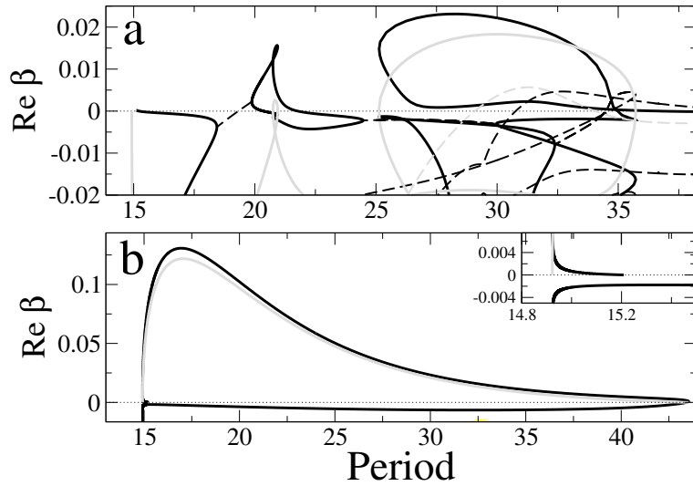
Fig. 19. The dominant eigenvalues \beta along the n = 2 primary branch for Ma=3.5 , Bi=0.5 , Bo=0.5 and \alpha = 0.135 (shown as a gray dashed line in Fig. 12). The solid (dashed) lines indicate real (complex) eigenvalues. The gray (black) lines refer to symmetry-preserving (-breaking) perturbations. Panel (a) refers to the upper part of the branch, while (b) refers to the lower part, above and below the saddle-node bifurcation at L \approx 14.92 , respectively.
