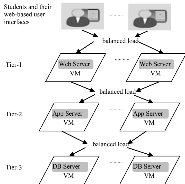
Figure 2. Our hypothetical 3-tier, cloud-based distributed system that is used to accomplish our tutorial scenario.
