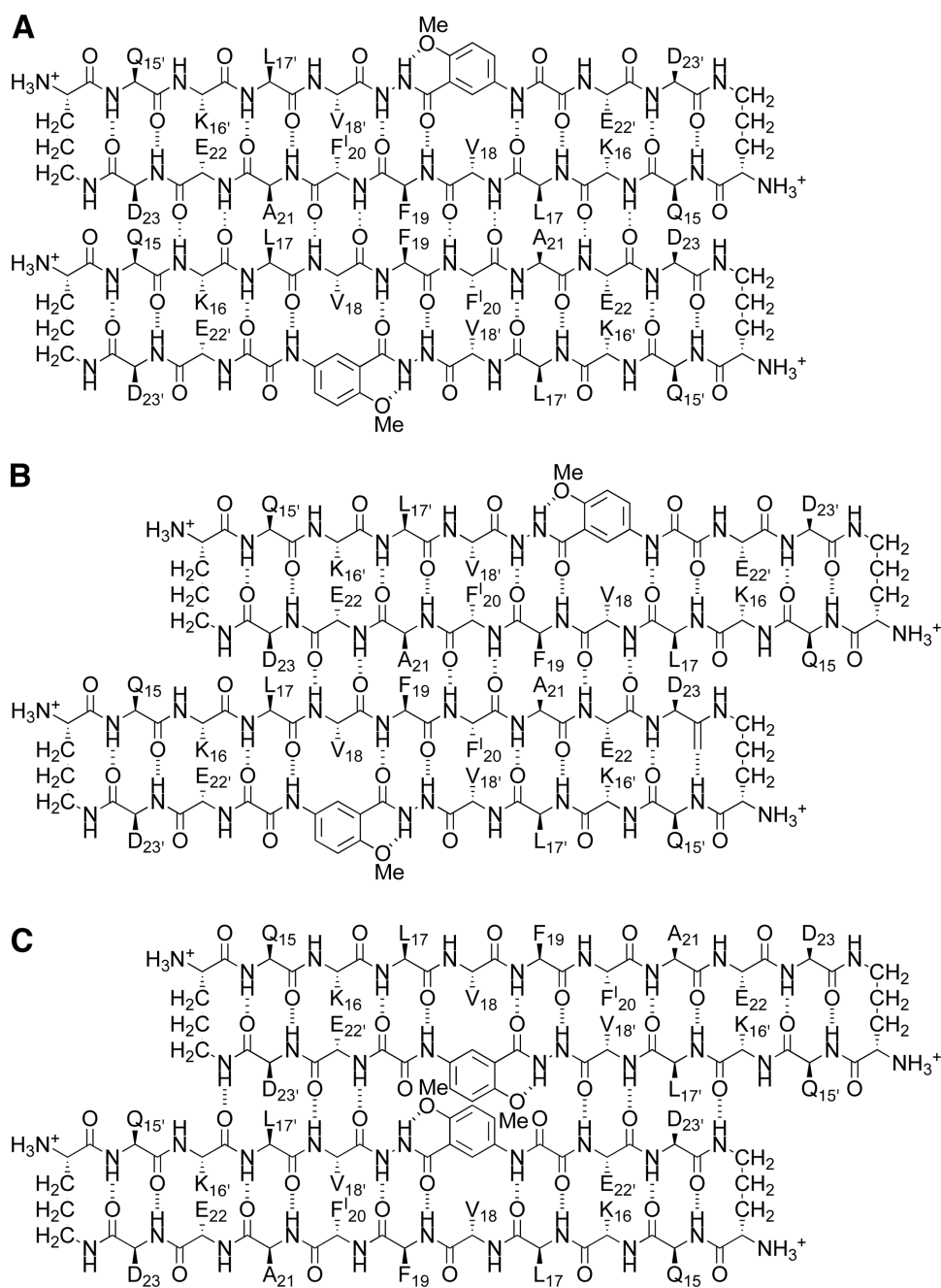
Figure 9. Interfaces between A\beta_{15-23} observed in the solid state and in solution. (A) Interface between monomer subunits within the dimer of macrocyclic \beta -sheet peptide 3 in the solid state. (B) Interface between monomer subunits within the dimer of macrocyclic \beta -sheet 3 in aqueous solution. (C) Interface between the dimers of macrocyclic \beta -sheet 3 in the solid state. In (A) and (B) the interface occurs between the A\beta_{15-23} peptide strands; in (C) the interface occurs between the A\beta_{15-23} hybrid strands.
