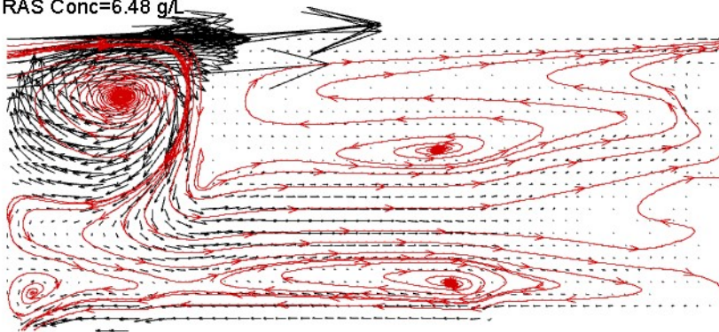
Figure 27- (a) Simulated velocities and solids distribution and (b) streamline after geometry modification (simulation 24).
