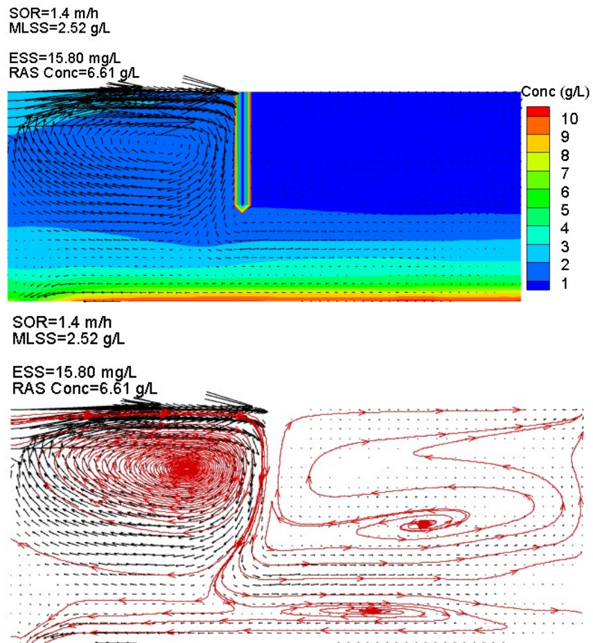
Figure 21- (a) Simulated velocities and solids distribution and (b) streamline before geometry modification (simulation 8).
