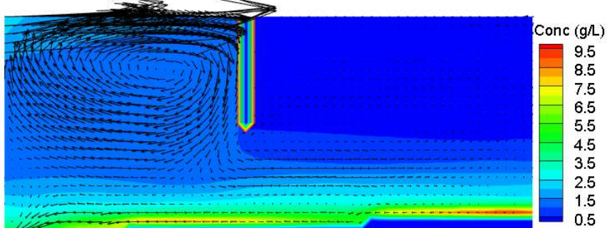
Figure 5- (a) Simulated velocities and solids distribution (Simulation 3).
