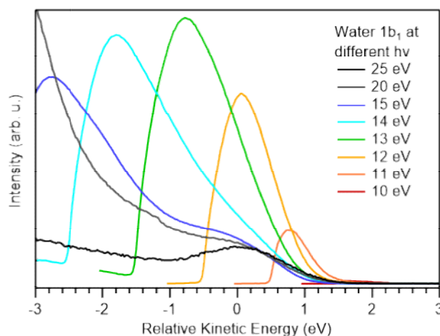
Figure SI-6: Photoemission spectra from liquid water obtained for photon energies of 10-25 eV, which covers energies above and below VIE_{1b_1(l)} ( = 11.3 eV); the figure is based on the same data as Fig. 3 in the main text. As before, all spectra are shifted so as to compensate for the difference in photon energy according to h\nu - VIE_{1b_1(l)} ( VIE_{1b_1(l)} = 11.3 eV). Unlike in Fig. 3, LET intensities are not clipped but rather displayed to yield the approximate relative intensities. For that, spectral intensities have been adjusted for photon flux and for (very approximate) changes in analyzer transmission; the latter is found to be sufficient for our qualitative analysis.
