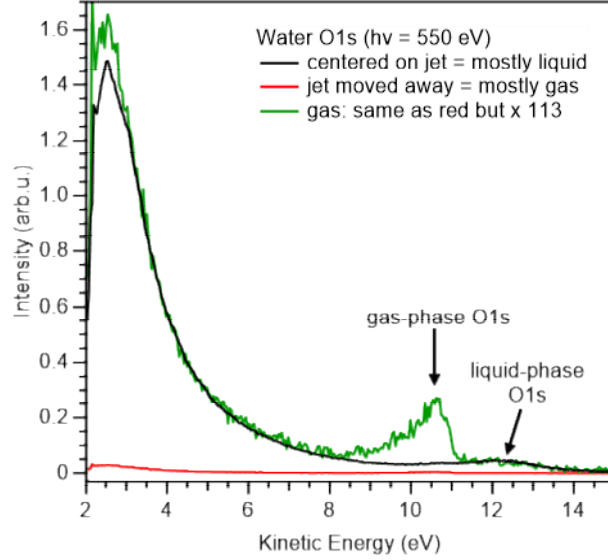
Figure SI-8: Photoemission spectra from liquid and gas-phase water measured at 550 eV photon energy using TOF spectroscopy, exhibiting the respective O 1s photoelectron peaks and LETs. The black curve shows the signal when the overlap between the liquid jet and the X-ray focus is optimized. The red curve was measured when the jet position was shifted sufficiently so that the X-ray spot has almost no overlap with the liquid jet, resulting in almost exclusive ionization of the surrounding gas-phase molecules. The green curve shows the red curve multiplied by a factor 113 which yields matching LET spectra. We find that the small contribution from the liquid phase essentially yields a scaled-down liquid water photoemission spectrum, implying that there is no LET signal generated in the gas phase. Spectra were measured with the magnetic bottle set-up described in conjunction with Fig. 4 of the main text. The asymmetry of the O 1s gas-phase peak results from both vibrational excitations 5 and asymmetric peak broadening due to post-collision interactions.
