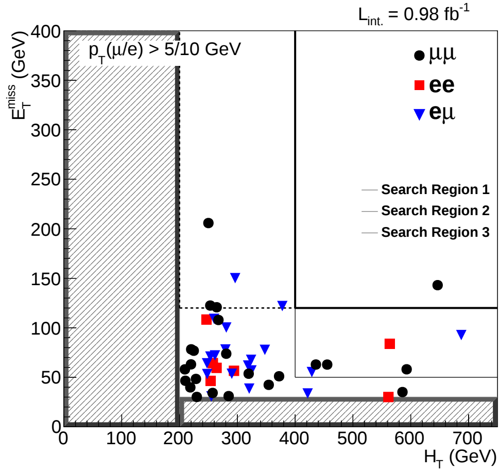
Figure 7.3: Distribution of events in the H_T - E_T plane passing the analysis selections for the inclusive dilepton control region. From [45]
