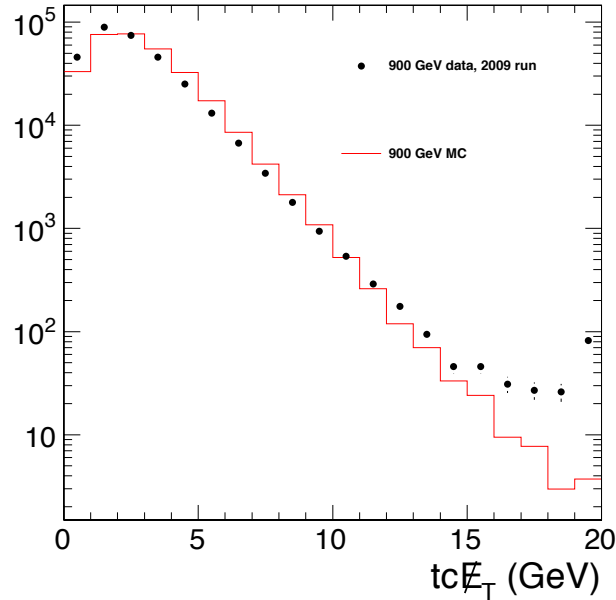
Figure 2.11: Distribution of tc\cancel{E}_T in data and MC at the start of the commissioning of 2009 data.
