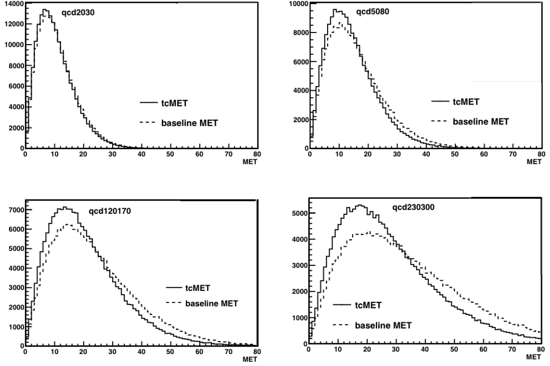
Figure 2.9: Comparison of tc\cancel{E}_T and corrected \text{calo}\cancel{E}_T . Four different \hat{p}_T ranges are shown, where qcdXY refers to the lower value, X, and upper value, Y, of the \hat{p}_T interval. In all cases, tc\cancel{E}_T improves both the tail and resolution of the \cancel{E}_T distribution with the degree of improvement increasing with \hat{p}_T .
