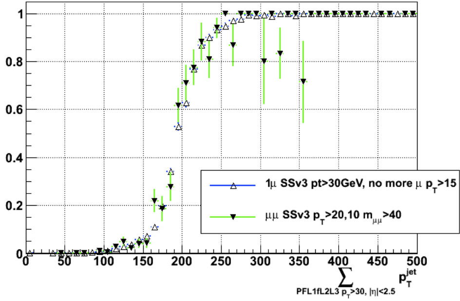
Figure 6.2: H_T trigger turn-on curves for the HT150/HT160 triggers as a function of the L1FastL2L3-corrected particle-flow jets. The jets are required to pass a selection of p_T > 30 GeV and |\eta| < 2.5 . The curve measured for the single-muon+ H_T trigger in event with only one muon (open triangles) represent the efficiency in W +jets events. The curve measured for the dimuon H_T trigger in events with two muons (filled triangles) represents the efficiency in Z +jets events.
