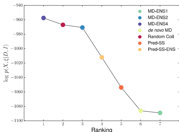
Figure 8: \log p(X, \xi | D, I) evaluated for X equal to 7 different ensembles for the A \beta 42 monomer shown in Figure 7 using both J-coupling and chemical shift data, but artificially reducing back-calculation uncertainties by a factor of 3.
