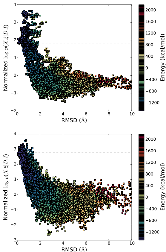
Figure 2: \log p(X, \xi \vee D, I) vs. RMSD for ~25,000 misfolded structures for 1L2Y using a uniform prior for (a) OISD and (b) EISD. Dotted black lines represent the fit-to-data probability of the native structure. All probabilities were normalized so the set had a mean of 0 and a variance of 1 (for easier comparison between schemes).
