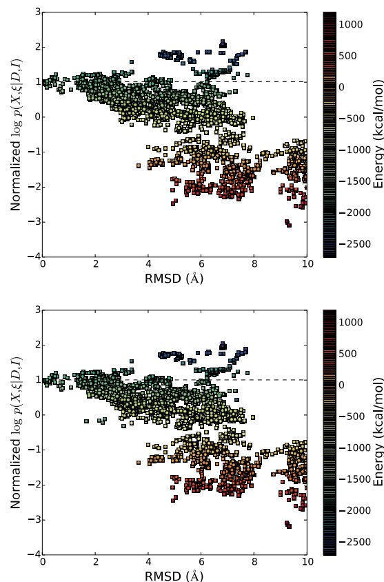
Figure 4: \log p(X, \xi \vee D, I) vs. RMSD for ~25,000 structures for 1GH9 for (a) OISD and (b) EISD using a Boltzmann prior. See Figure 2 caption for further details.
