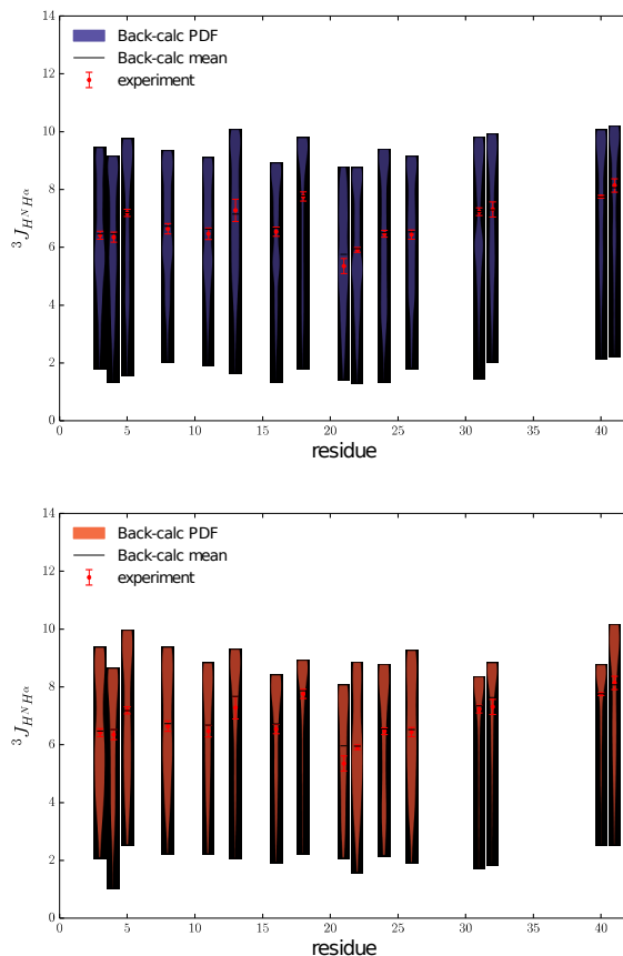
Figure 7: Gaussian Kernel Density Estimation of the probability distributions of back-calculated J-coupling constants from (a) MD-ENS4 and (b) Pred-SS. Wider areas represent higher probabilities.
