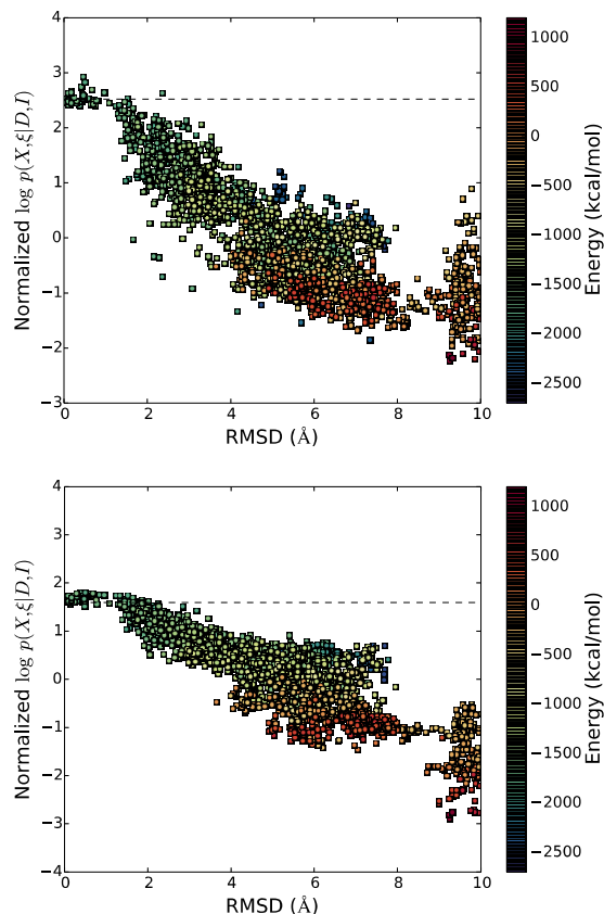
Figure 3: \log p(X, \xi \vee D, I) vs. RMSD for ~25,000 misfolded structures for 1GH9 for (a) OISD and (b) EISD using a uniform prior. See Figure 2 caption for further details.
