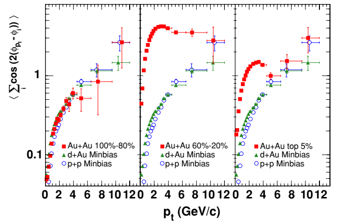
FIG. 12. (Color online) Charged-hadron azimuthal correlations vs. p_t in Au+Au collisions (squares) as a function of centrality (peripheral to central from left to right) compared to minimum bias azimuthal correlations in p+p collisions (circles) and d+Au collisions (triangles). The Au+Au and p+p data are from Ref. [6].
