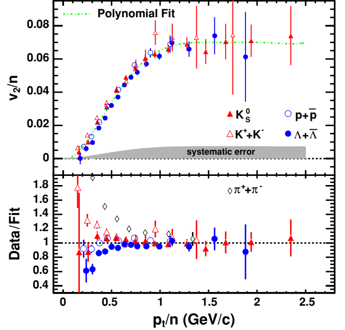
FIG. 33. (Color online) (Top panel) Identified particle v_2 from minimum bias collisions. The vertical axis and horizontal axis have been scaled by the number of constituent quarks ( n ). Pions are not plotted. A polynomial curve is fit to the data. The possible systematic error is indicated by the gray band. (Bottom panel) The ratio of v_2/n to the fitted curve.
