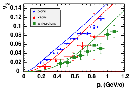
FIG. 6. (Color online) v_2\{4\} vs. p_t for identified particles in the 20–60% centrality range. The solid lines are hydrodynamic calculations [31].
