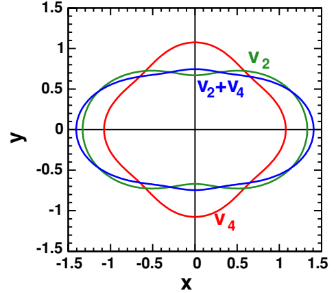
FIG. 23. (Color online) A polar graph of the distribution 1 + 2v_2 \cos(2\phi) + 2v_4 \cos(4\phi) , where \phi is the azimuthal angle relative to the positive x axis. Plotted are the distributions for v_2 = 16.5\% showing the waist, v_4 = 3.8\% having a diamond shape, and both coefficients together.
