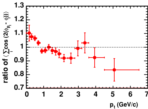
FIG. 14. (Color online) The ratio of the scalar product from the Au side ( -1.0 < \eta < -0.5 ) to that from the deuteron side ( 0.5 < \eta < 1.0 ) vs. p_t from minimum bias collisions.
