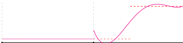
Figure 1.3: Polynomial basis from Figure 1.2 along with a discontinuous function.
