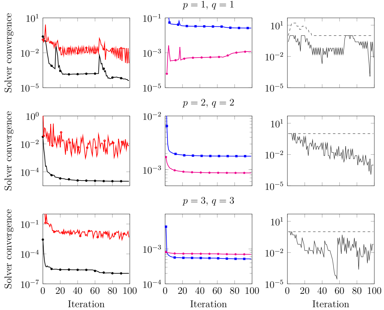
Figure 4.16: Convergence of the DG residual \|\mathbf{r}(\mathbf{u}, \mathbf{x})\| ( \bullet ), enriched DG residual \|\mathbf{R}(\mathbf{u}, \mathbf{x})\| ( \bullet ), optimality condition \|\mathbf{c}(\mathbf{u}, \mathbf{x})\| ( \bullet ), mesh distortion \|\kappa \mathbf{R}_{\text{msh}}(\mathbf{x})\| ( \bullet ) and control of the regularization parameter (---) and step size (—) for the tracking method applied to solve the supersonic flow around the NACA airfoil. For this difficult problem, the convergence of the KKT system is not as clean as the other problems and relies heavily on the line search; however, the solver still tracks the shocks and returns an accurate flow as seen from the solution plots (Figures 4.14-4.15). The spikes in the KKT conditions for p = q = 1 are due to element collapses.
