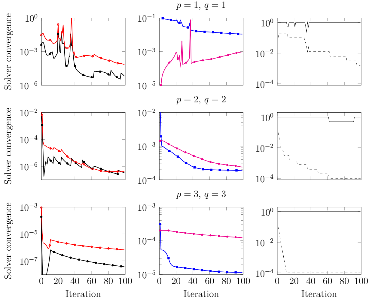
Figure 4.10: Convergence of the DG residual \|\mathbf{r}(\mathbf{u}, \mathbf{x})\| (—●—), enriched DG residual \|\mathbf{R}(\mathbf{u}, \mathbf{x})\| (—■—), optimality condition \|\mathbf{c}(\mathbf{u}, \mathbf{x})\| (—●—), mesh distortion \|\kappa \mathbf{R}_{\text{msh}}(\mathbf{x})\| (—●—) and control of the regularization parameter (---) and step size (—) for the tracking method applied to the inviscid Burgers' equation.
