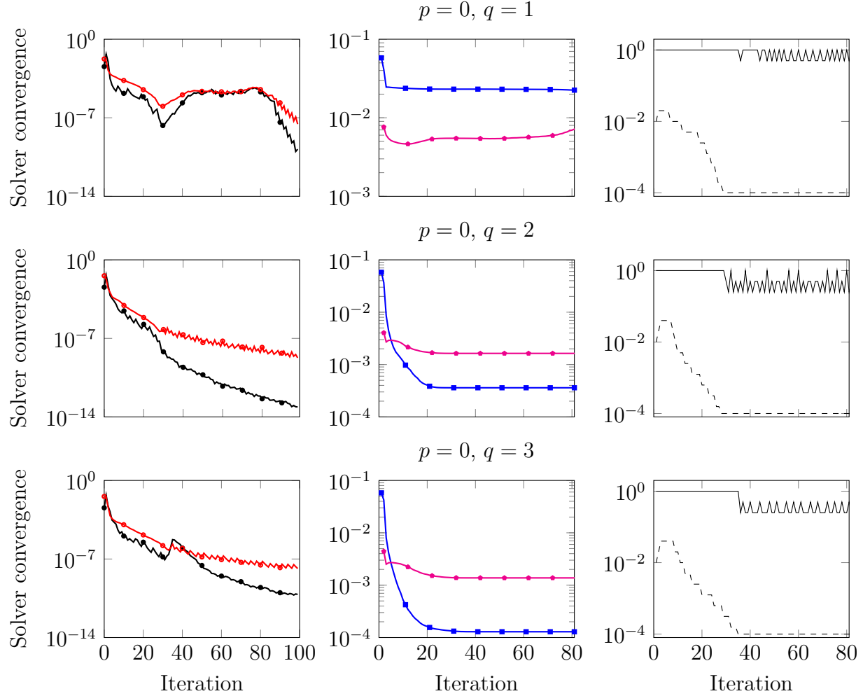
Figure 4.5: Convergence of the DG residual \|\mathbf{r}(\mathbf{u}, \mathbf{x})\| (—●—), enriched DG residual \|\mathbf{R}(\mathbf{u}, \mathbf{x})\| (—■—), optimality condition \|\mathbf{c}(\mathbf{u}, \mathbf{x})\| (—○—), mesh distortion \|\kappa \mathbf{R}_{\text{msh}}(\mathbf{x})\| (—●—), and control of the regularization parameter (---) and step size (—) for the tracking method applied to the advection equation with the trigonometric shock. Even though Newton convergence is not achieved, the proposed solver converges the KKT system to tight tolerances in a reasonable number of iterations.
