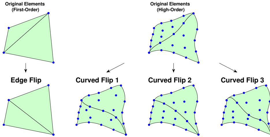
Figure 6.2: Only one possible flip for straight-sided elements, but many possible flips in the high-order setting.
