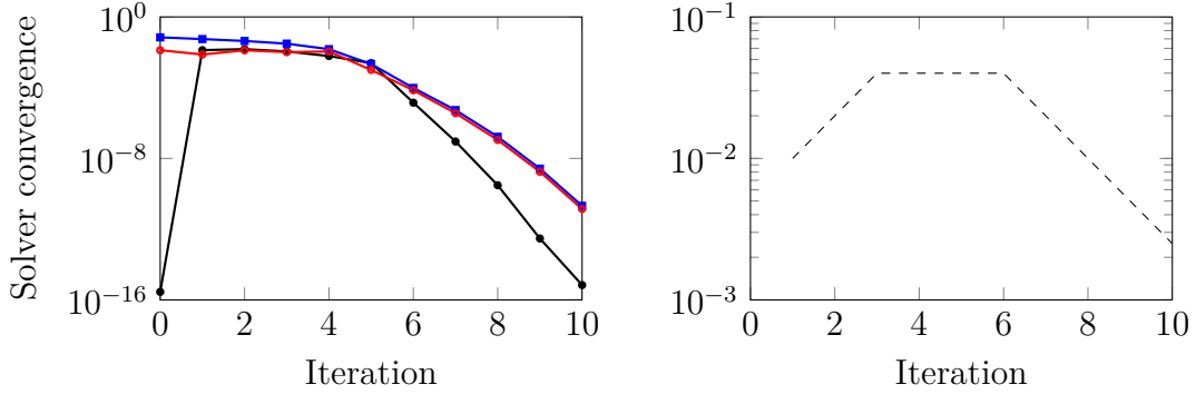
Figure 4.3: Convergence of the DG residual \|\mathbf{r}(\mathbf{u}, \mathbf{x})\| ( \blacktriangleleft ), enriched DG residual \|\mathbf{R}(\mathbf{u}, \mathbf{x})\| ( \blacksquare ), optimality condition \|\mathbf{c}(\mathbf{u}, \mathbf{x})\| ( \bullet ), and control of the regularization parameter (---) for the tracking method applied to the advection equation with a straight shock (constant advection field). For this simple problem, Newton-like convergence is achieved.
