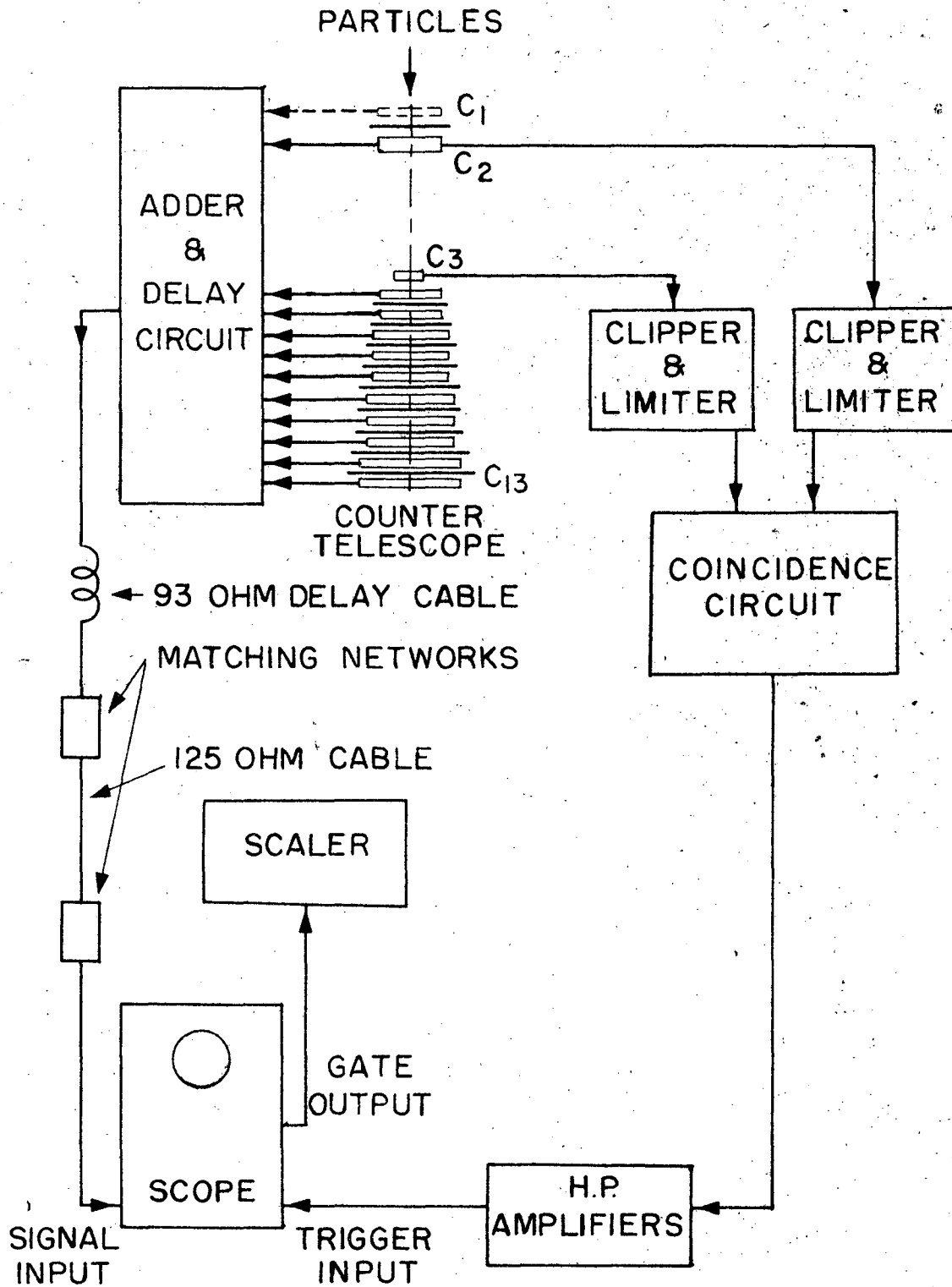
ELECTRONICS BLOCK DIAGRAM
