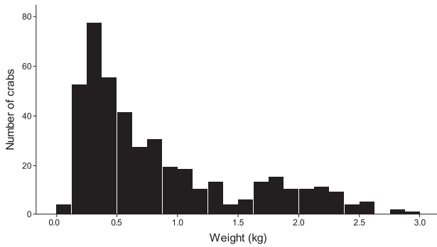
FIG. 3 Weight distribution of the 436 coconut crabs captured in Tanzania.
