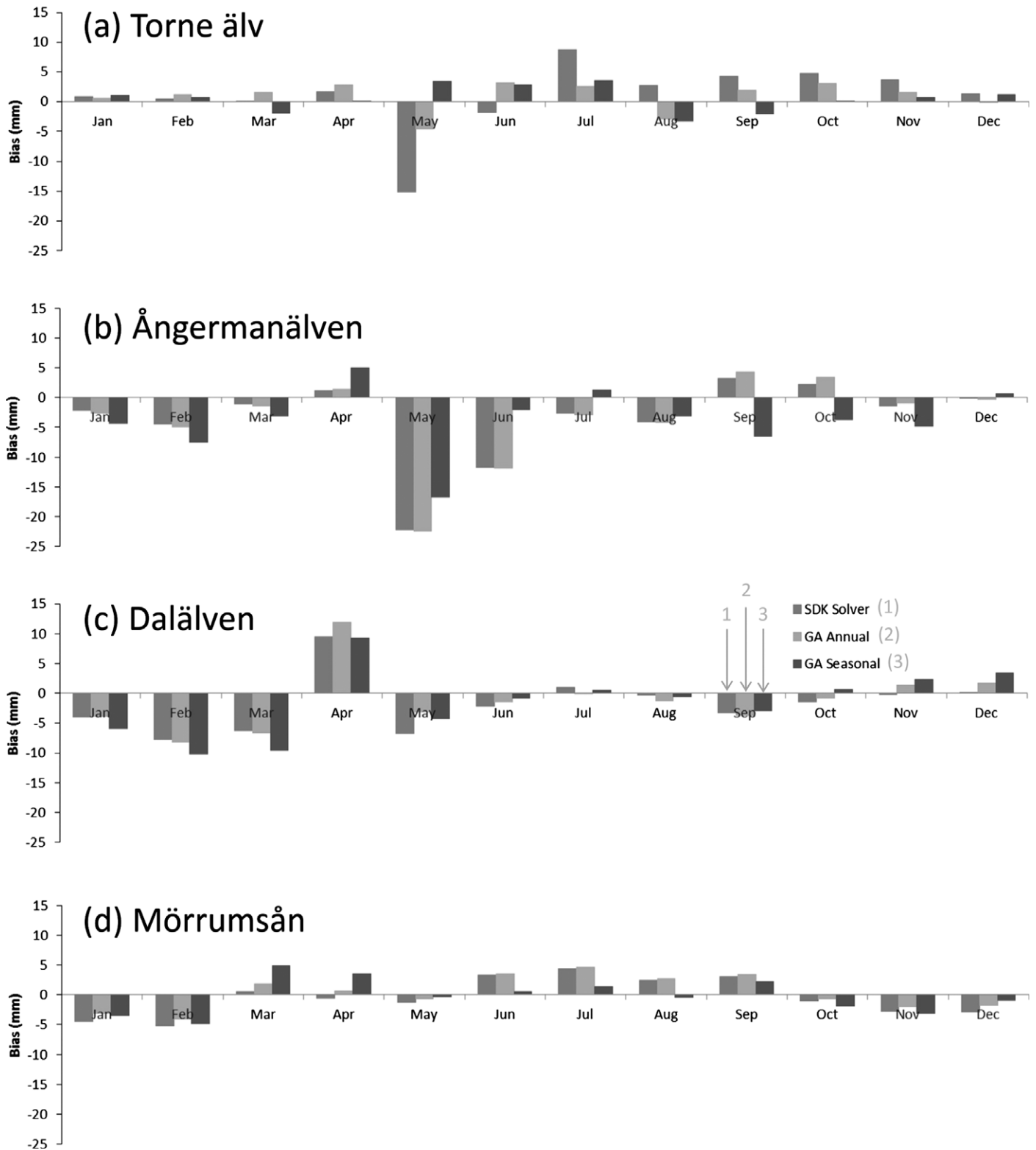
FIGURE 6. Monthly Variations in Model Bias for (a) Torne älv, (b) Ångermanälven, (c) Dalälven, and (d) Mörrumsån for the Catchment Simulation Model When Calibrated Using the SDK Solver as in Mörtz et al. (2007) or the Genetic Algorithm Procedure without (and with) Seasonal Parameterization of the Subsurface Flow Representation.
