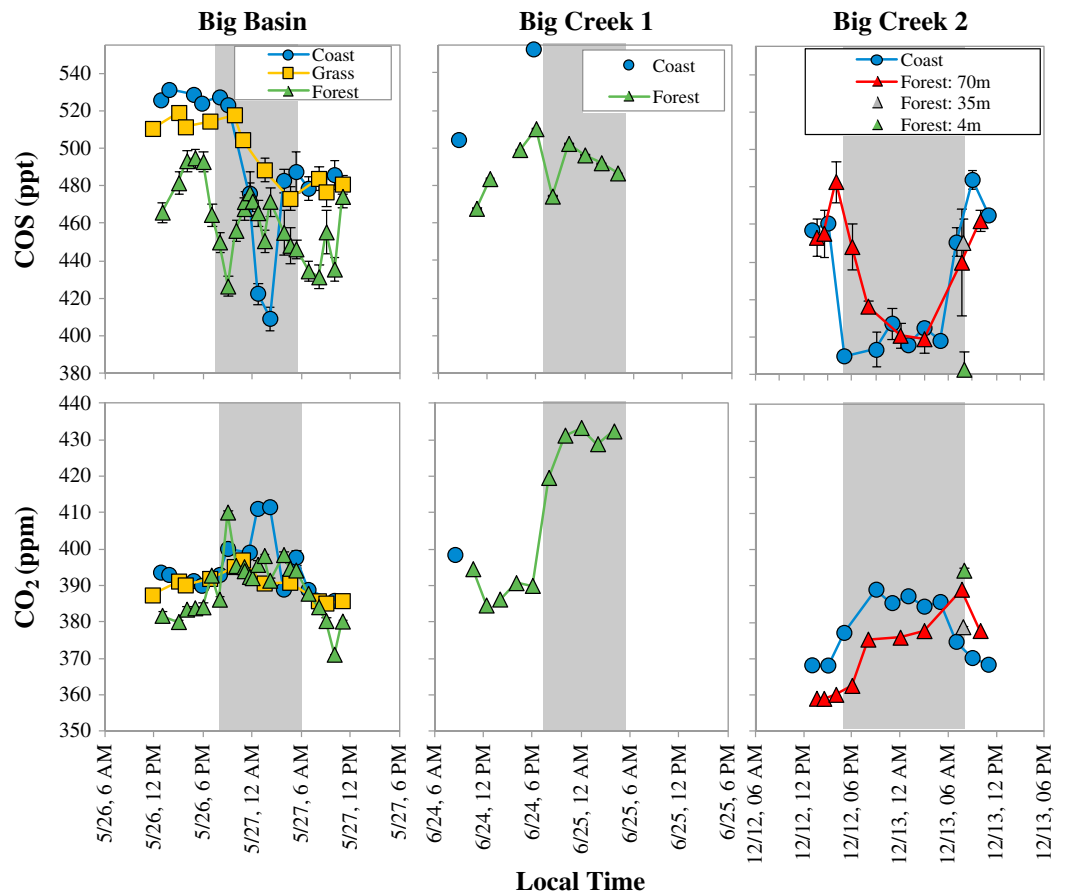
Figure 2. Measurements of COS and CO 2 in ambient air from three field campaigns (Big Basin, Big Creek 1, and Big Creek 2) at coast redwood and adjacent sites. All sample heights are near-surface (2–4 m aboveground level) except for a subset of the forest site samples during the Big Creek 2 campaign, which included samples at 70 m and 35 m aboveground level. Measurement uncertainties are the standard deviation of multiple measurements on each flask; many symbols obscure the error bars. Site locations in Figure 1c and Table 1. The gray shading is nighttime.
