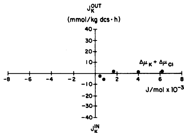
FIGURE 5. Correspondence between the magnitude and direction (sign) of NEM-induced net K flux and the force driving K/H exchange ( \Delta\mu_K - \Delta\mu_H ) or KCl cotransport ( \Delta\mu_K + \Delta\mu_{Cl} ). The cells were treated with 100 \mu M DIDS in order to inhibit the anion exchanger and permit independent variations in \Delta\mu_H and \Delta\mu_{Cl} . The force driving KCl cotransport ( \Delta\mu_K + \Delta\mu_{Cl} ) was then varied over a range of 6,000 J/mol while the driving force for K/H exchange was held at zero. These data are representative of three identical experiments. While not shown in the figure, a control that held the force driving KCl cotransport and that driving K/H exchange at \sim 7,000 J/mol resulted in a net K loss of 32 meq in 1 h (see also the legend to Fig. 3).
