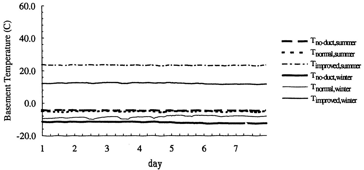
FIGURE 5. Comparison of T_{basement} between the no-duct, normal ducts, and improved duct cases for heating and cooling. The perfect duct case is not shown because T_{base,perfect} = T_{base,no-duct} .
