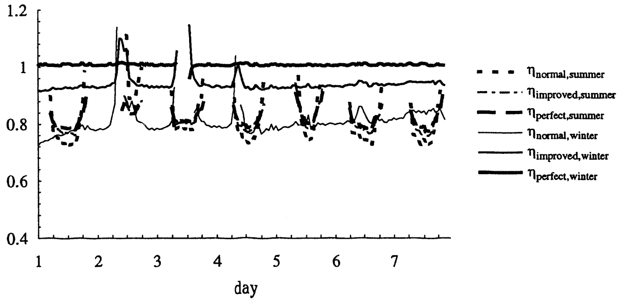
FIGURE 6. Comparison of \eta_{dist} between the normal, improved, and perfect duct cases for heating and cooling.
