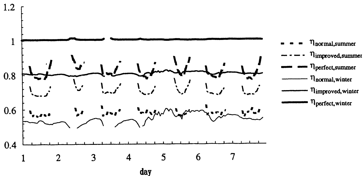
FIGURE 7. Comparison of \eta_{\text{nominal}} between the normal, improved, and perfect duct cases for both heating and cooling.
