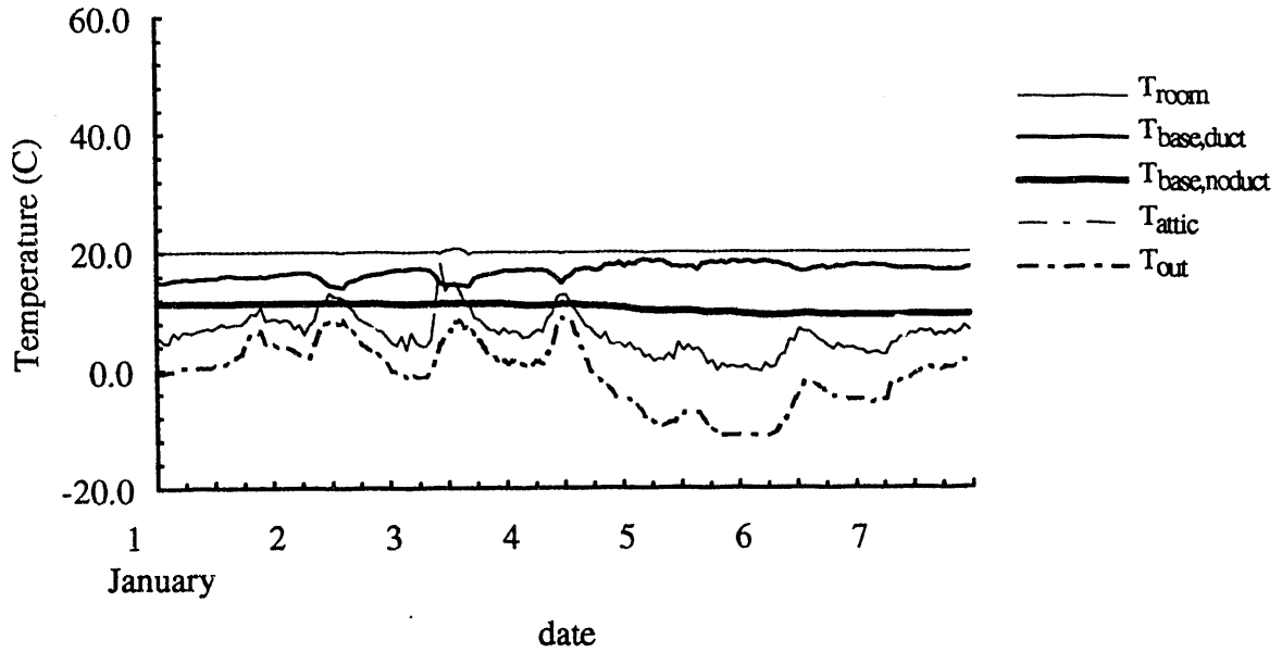
FIGURE 3. Zone temperatures for Washington with normal ducts for January 1-7.
