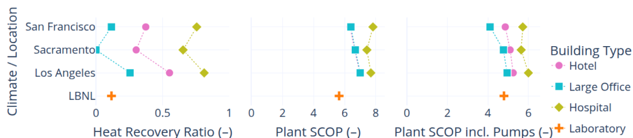
Figure 9: Sensitivity of the Heat Recovery Rate (left), Plant Seasonal Coefficient of Performance (SCOP) of primary generating equipment only (middle), and SCOP with pumps (right) across California climate zones (San Francisco, Sacramento, Los Angeles) and representative building types for the nominal thermal storage size (3h of peak load).
