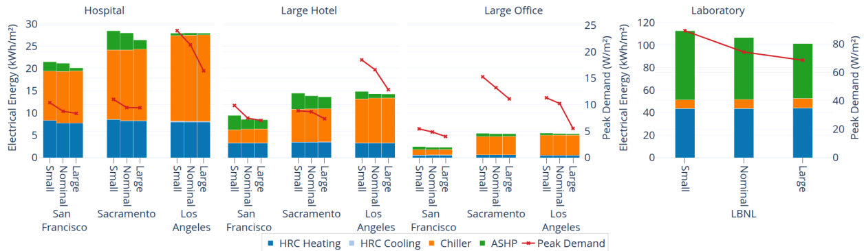
Figure 10: Operational trade-offs of equipment sizing rules, comparing Small (15-minute), Nominal (3-hour), and Large (8-hour) TES capacities across three building types for the different climates and building types on the left side, and real laboratory building on the right side. Stacked bars represent annual electrical energy use by equipment type, while the red line indicates peak electrical demand.
