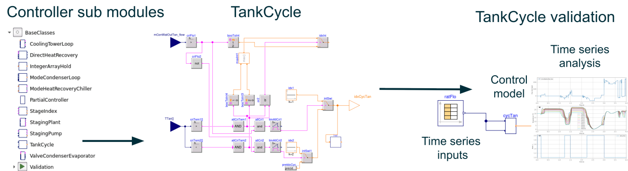
Figure 2: Controls validation example TankCycle sub module.
