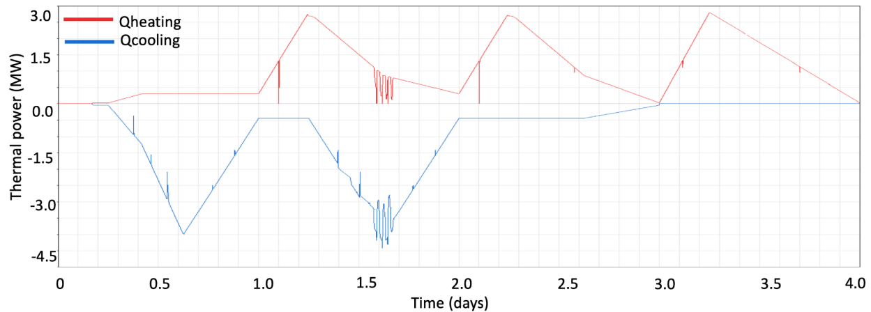
Figure 3: Heating and cooling loads of the four-day plant simulation used for control validation.
