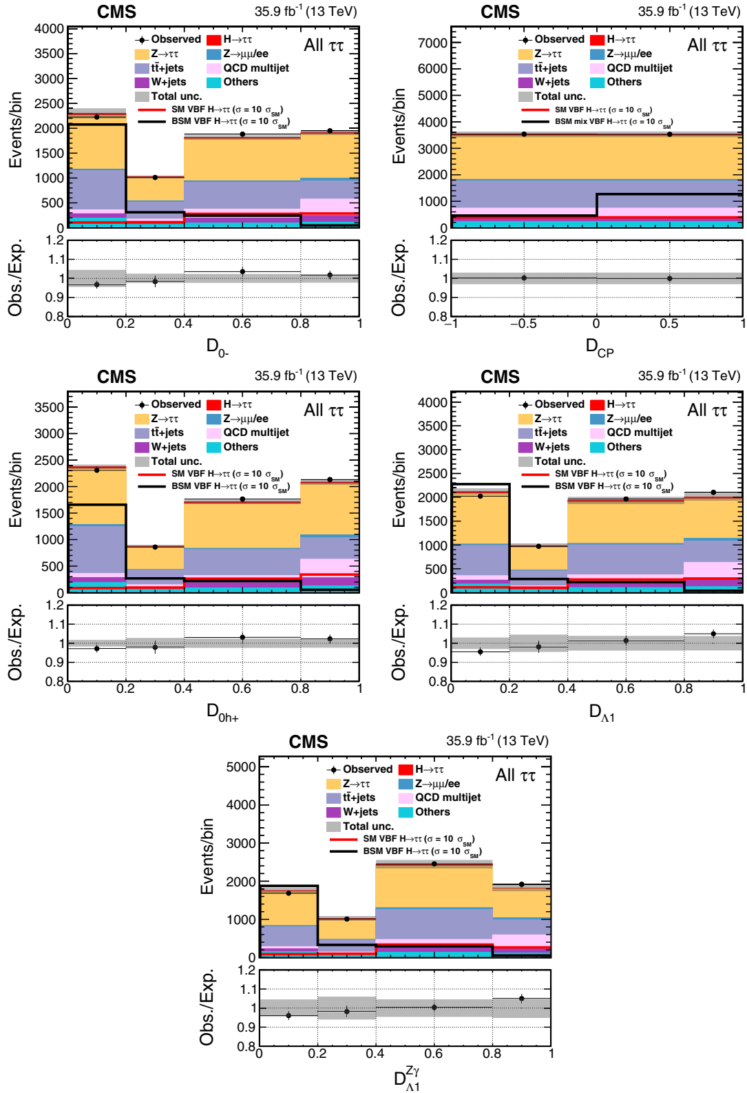
FIG. 5. The distribution of D_{0-} , D_{CP} , D_{0h+} , D_{\Lambda 1} , and D_{\Lambda 1}^{Z\gamma} in the VBF category. All four decay channels, e\mu , e\tau_h , \mu\tau_h , and \tau_h\tau_h , are summed. The BSM hypothesis depends on the variable shown; it corresponds to f_{a3} \cos(\phi_{a3}) = 1 for the D_{0-} (upper left) distribution, the maximal mixing in VBF production (“BSM mix,” corresponding to f_{a3} \cos(\phi_{a3}) = 0.013 ) for the D_{CP} distribution (upper right), f_{a2} \cos(\phi_{a2}) = 1 for the D_{0h+} distribution (middle left), f_{\Lambda 1} \cos(\phi_{\Lambda 1}) = 1 for the D_{\Lambda 1} distribution (middle right), and f_{\Lambda 1}^{Z\gamma} \cos(\phi_{\Lambda 1}^{Z\gamma}) = 1 for the D_{\Lambda 1}^{Z\gamma} distribution (lower). The expected D_{CP} distribution is always symmetric, unless a CP -violating effect is present in the signal.
