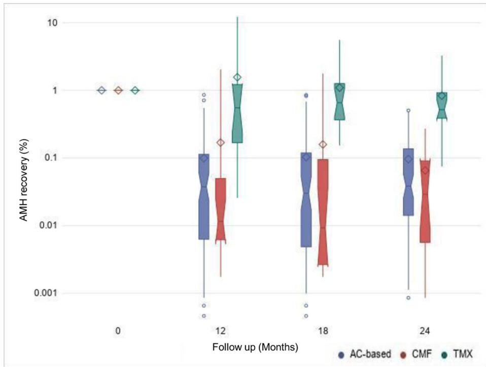
Fig. 3. Whisker Plot of representation of serum AMH recovery rates in women treated with AC-based, CMF and tamoxifen-only treatments during the 12-, 18- and 24-months follow-up. After a baseline assessment, 142 women were followed up for 24-months with serum AMH measurements either after the completion of chemotherapy or during tamoxifen-only treatment. AMH recovery was calculated by the ratio dividing follow up AMH values by the baseline value at each time point, where ratio=1 means full recovery. AMH recovery rate was similar between women who received treatment with AC-based and CMF chemotherapy regimens 12-, 18- and 24-months after the completion of chemotherapy. Tamoxifen treatment alone was associated with higher recovery rates compared with chemotherapy groups at 12-, 18- and 24-months follow-up. See Table 1S for summary statistics for each subgroup at different time points. AC Anthracycline and cyclophosphamide, CMF Cyclophosphamide, Methotrexate, 5-Fluorouracil, Tmx Tamoxifen 20 mg/day.
