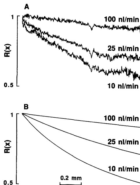
FIGURE 4. Dependence of the fluorescence intensity profile R(x) on luminal perfusion rate. (A) Experimental data at 50 mM bath Cl (solution 3). The lumen was perfused with solution 8 at the indicated rates. (B) Model calculations (Eqs. 6 and 8) with P_s = 2 \times 10^{-5} cm/s, P_f = 0.3 cm/s, \sigma_s = 1 , S = 0.0013 cm 2 /mm, C_i^o = 200 mM, C_p^o = 100 mM, C_i(0) = 300 mM, C_p(0) = 0 mM with V(0) as indicated.
