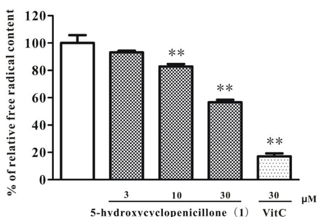
Figure 6. 5-hydroxycyclopicillone (1) scavenges DPPH free radicals in a concentration-dependent manner. Compound 1 or vitamin C (VitC) at indicated concentrations were added to 0.2 mM DPPH solution for 20 min. The concentration of DPPH free radicals was measured by evaluating the absorbance at 517 nm. Data are presented as the mean \pm SEM of three separate experiments; ** p < 0.01 vs. the control group (ANOVA and Dunnett's test).
